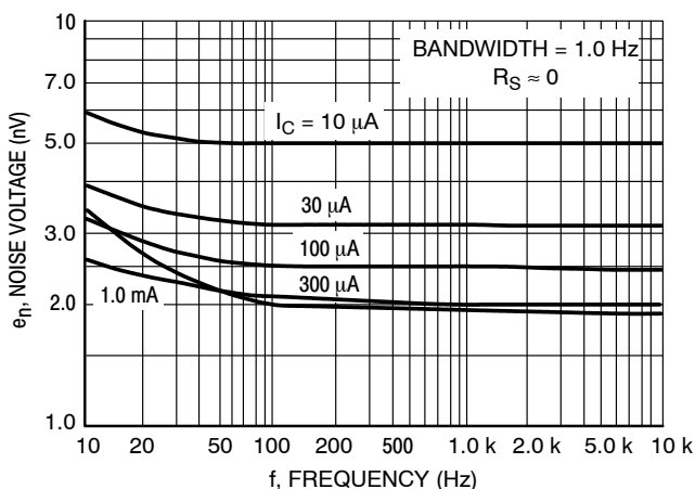
Figure 1. Noise Voltage
