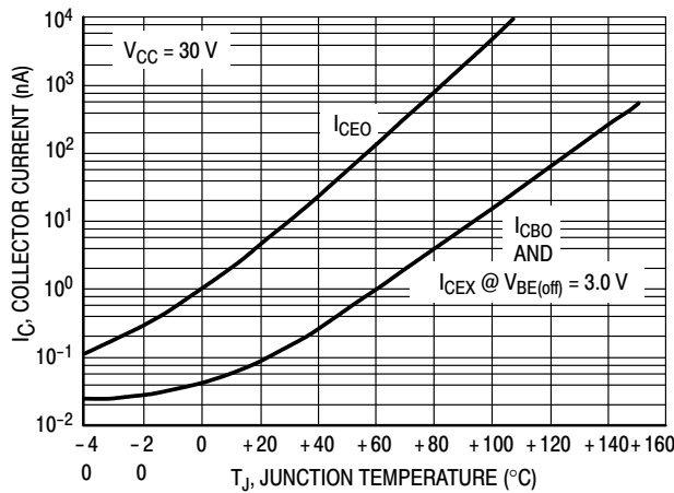
Figure 17. Typical Collector Leakage Current
