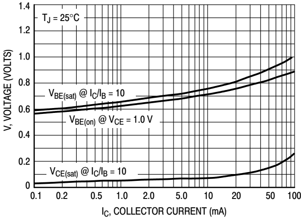
Figure 9. "On" Voltages
