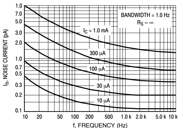
Figure 2. Noise Current
