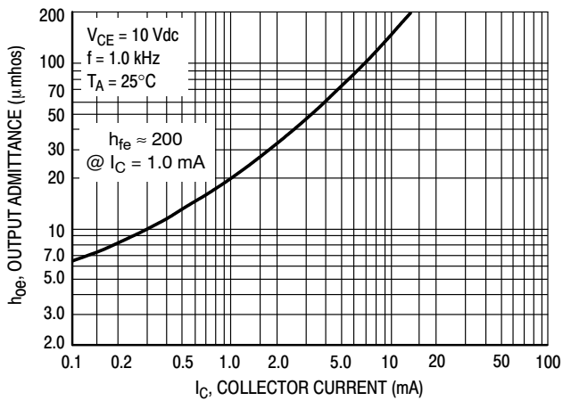
Figure 16. Output Admittance
