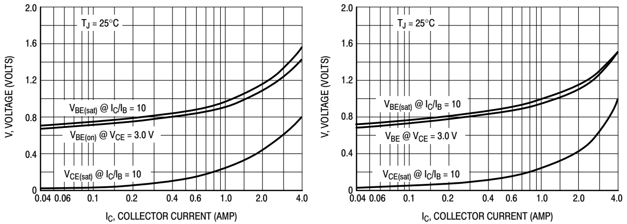
Figure 9. "On" Voltages
