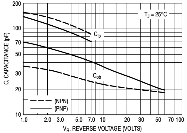
Figure 7. Capacitance
