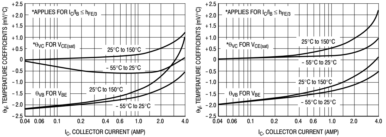
Figure 10. Temperature Coefficients
