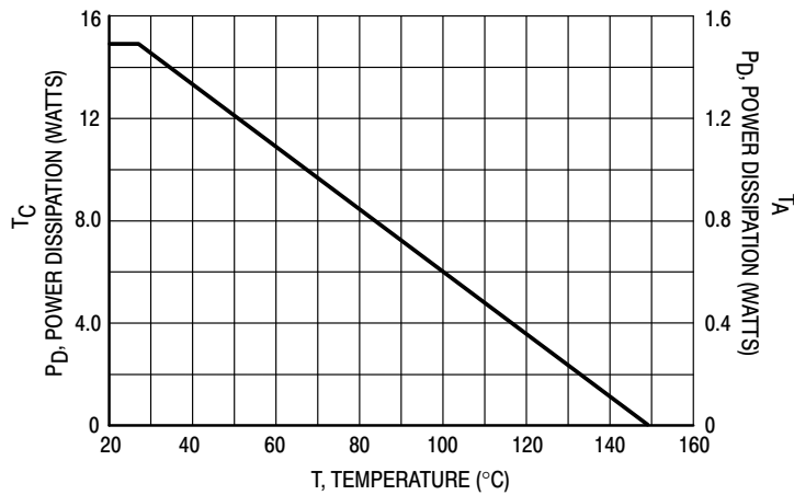
Figure 1. Power Derating
