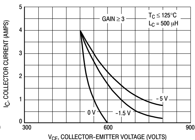
Figure 21. Reverse Bias Safe Operating Area
