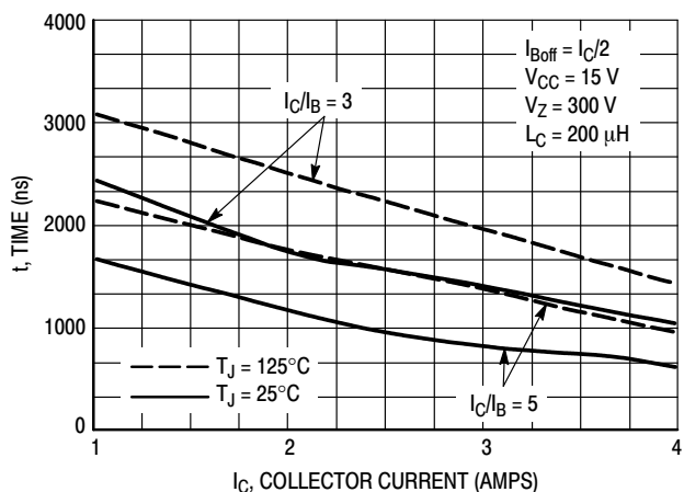
Figure 11. Inductive Storage Time, t_{si}
