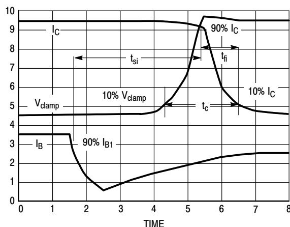
Figure 19. Inductive Switching Measurements
