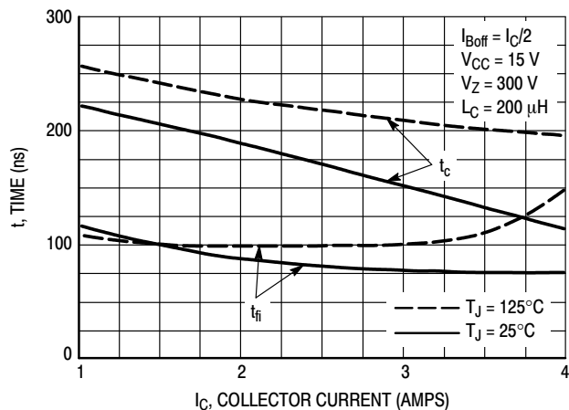
Figure 12. Inductive Storage Time, t_c & t_{fi} @ I_C/I_B = 3
