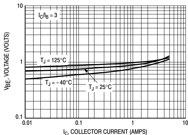
Figure 6. Base-Emitter Saturation Region
