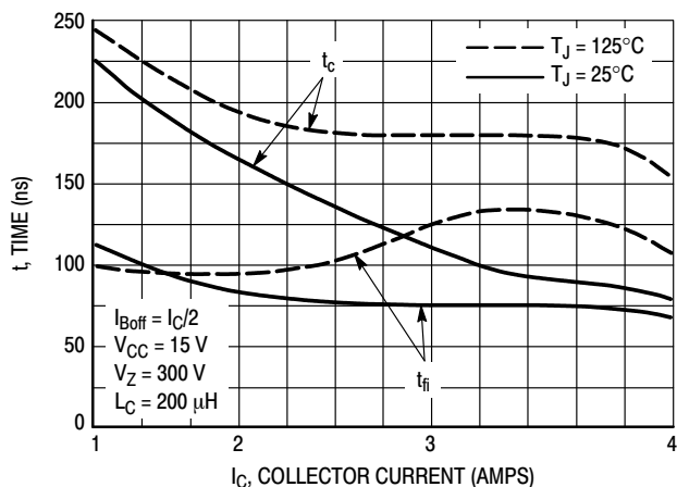
Figure 13. Inductive Switching, t_c & t_{fi} @ I_C/I_B = 5
