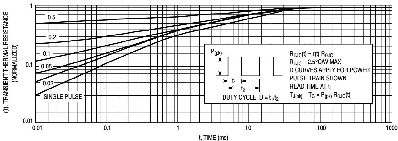
Figure 22. Typical Thermal Response ( Z_{\theta JC}(t) ) for BUH50
