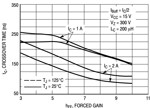
Figure 16. Inductive Crossover Time
