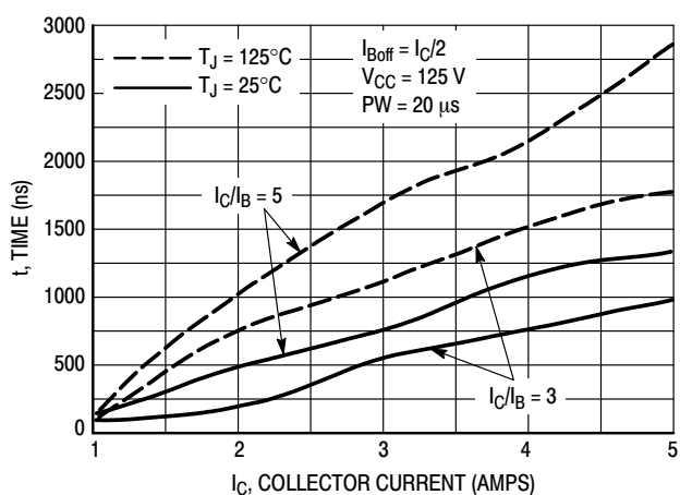
Figure 9. Resistive Switching, t_{on}
