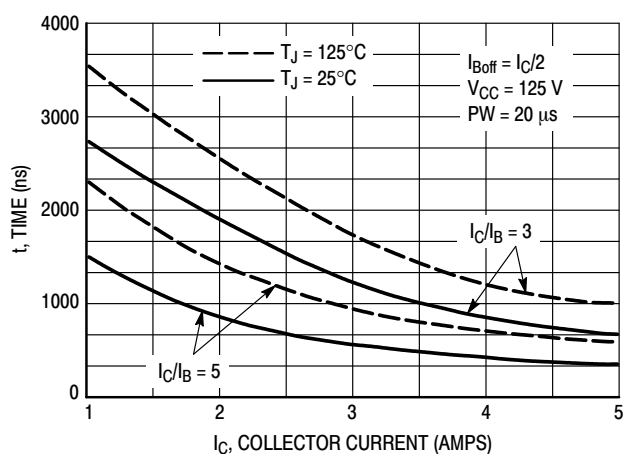
Figure 10. Resistive Switch Time, t_{off}
