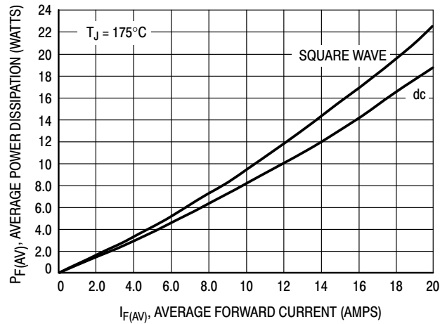
Figure 6. Power Dissipation, Per Leg
