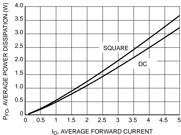
Figure 6. Power Dissipation
