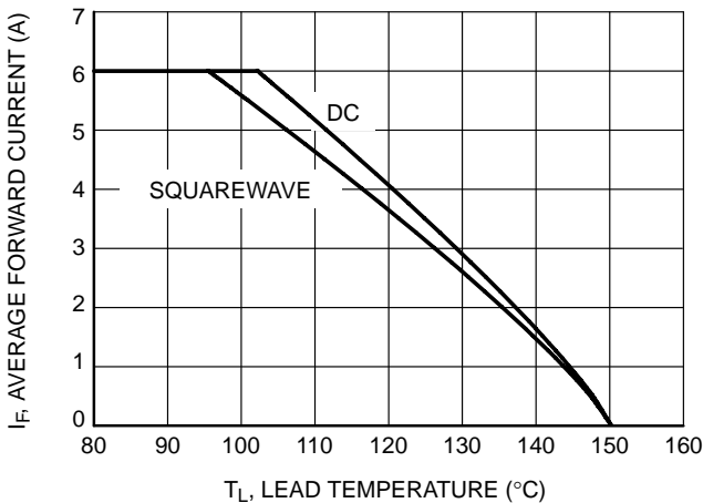
Figure 7. Derating Curve
