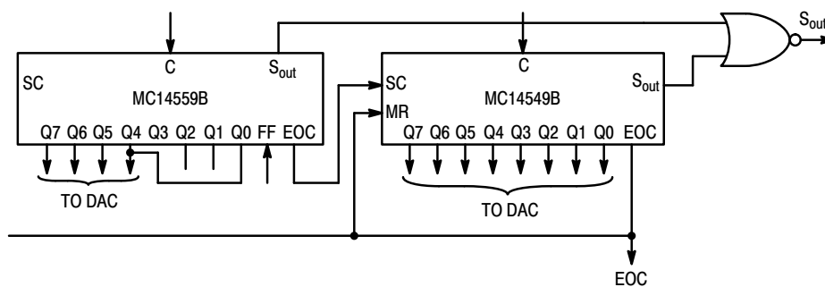
Figure 4. Continuously Cycling 12-Bit ADC
