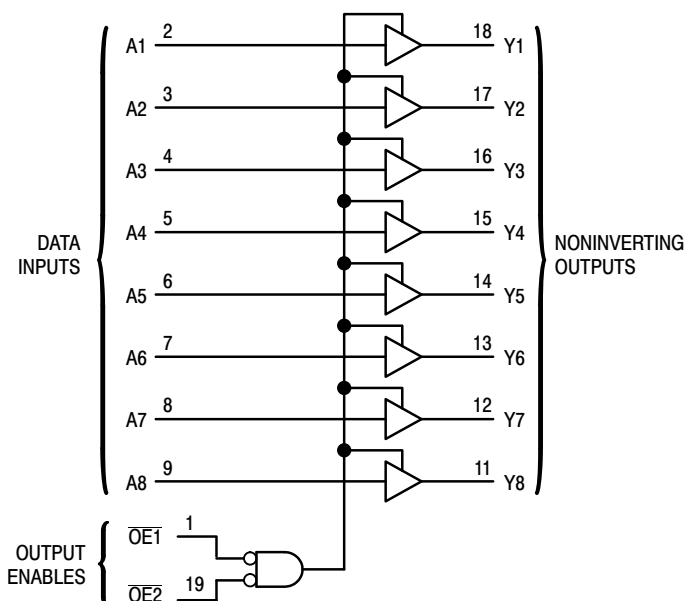
Figure 1. Logic Diagram
