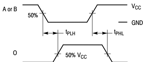
Figure 2. Switching Waveforms
