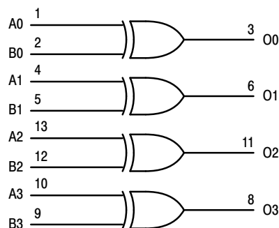
Figure 1. Logic Diagram
