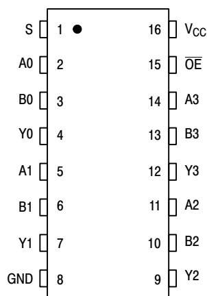
Figure 1. Pin Assignment
