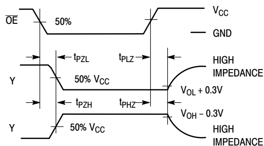
Figure 6. Switching Waveform
