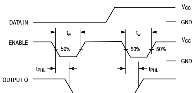
Figure 8. Switching Waveform
