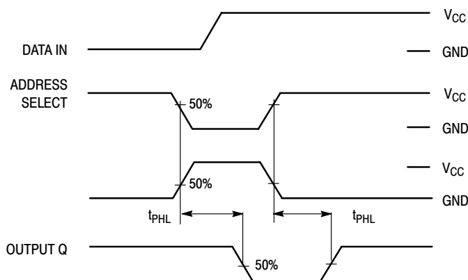
Figure 7. Switching Waveform
