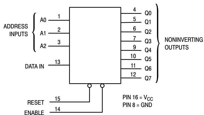
Figure 2. Logic Diagram
