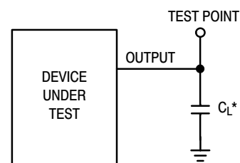
Figure 11. Test Circuit
