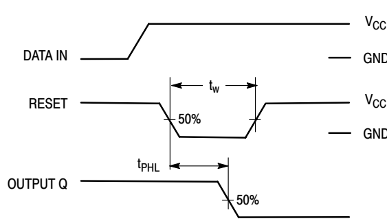
Figure 9. Switching Waveform
