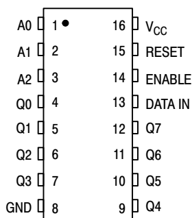
Figure 1. Pin Assignment
