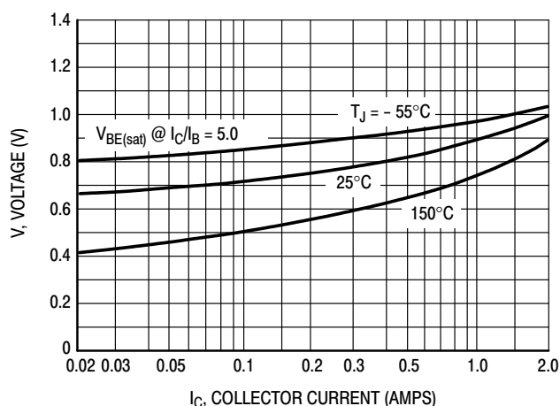
Figure 3. Base-Emitter Voltage
