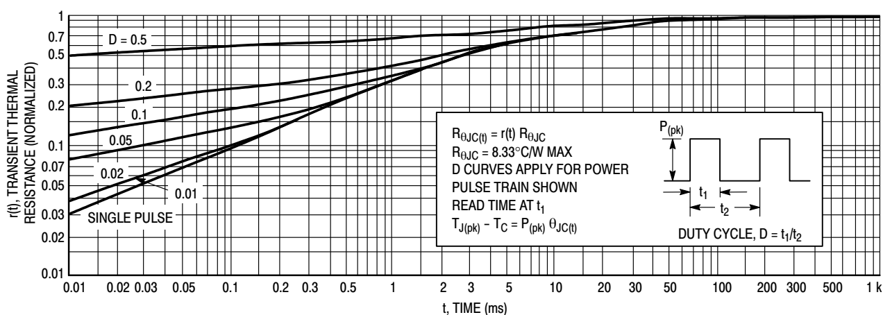
Figure 6. Thermal Response
