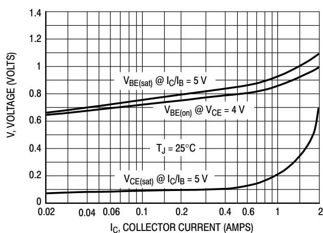
Figure 4. "On" Voltages
