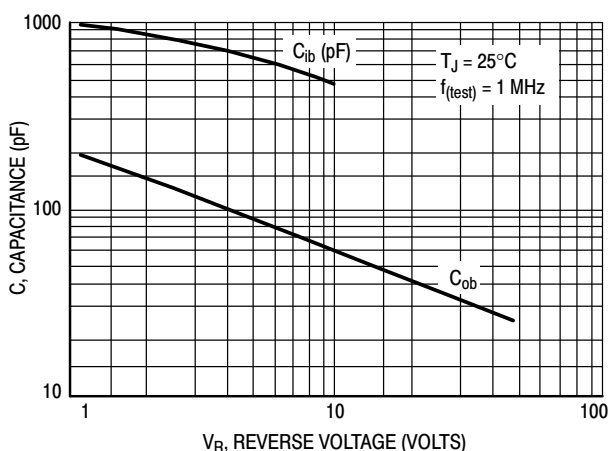
Figure 11. Capacitance
