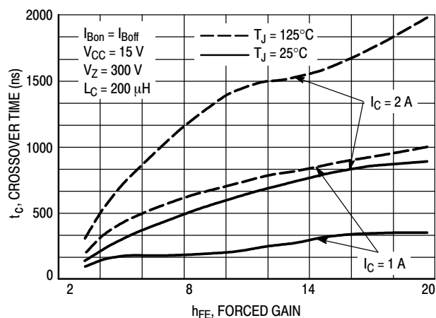
Figure 22. Inductive Crossover Time
