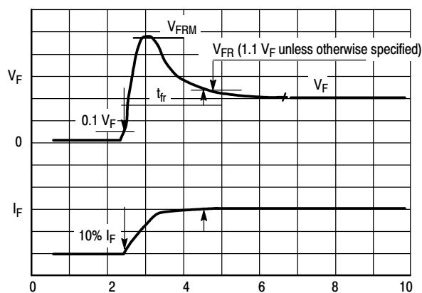
Figure 27. t_{fr} Measurements
