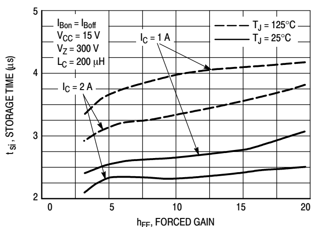
Figure 20. Inductive Storage Time
