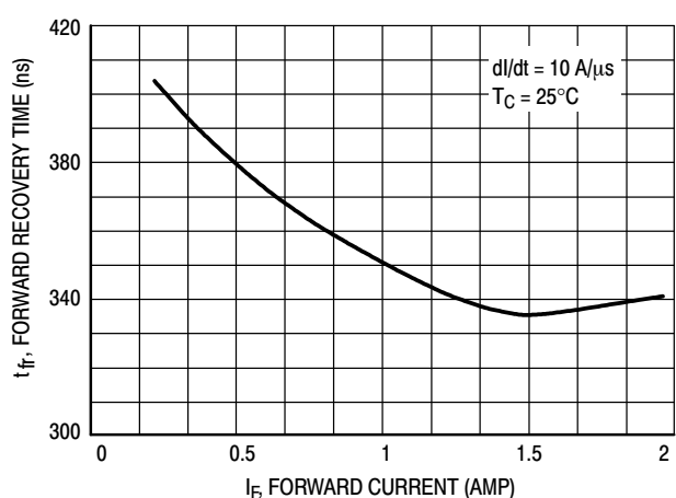
Figure 24. Forward Recovery Time, T_{FR}
