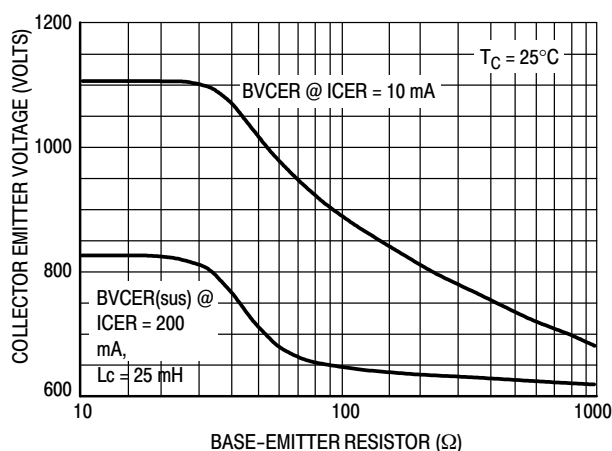
Figure 12. BV_{CEr} = f(R_{BE})
