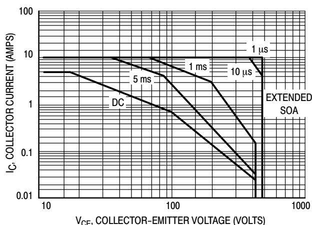
Figure 28. Forward Bias Safe Operating Area
