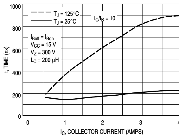
Figure 18. Inductive Switching Time, t_{fi} @ I_{C/I_B} = 10
