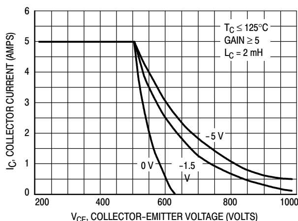
Figure 29. Reverse Bias Safe Operating Area
