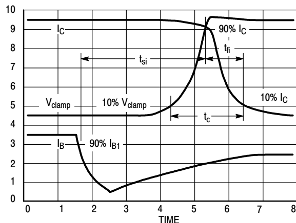
Figure 26. Inductive Switching Measurements
