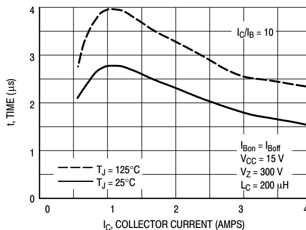
Figure 16. Inductive Storage Time, t_{si} @ I_{C/I_B} = 10
