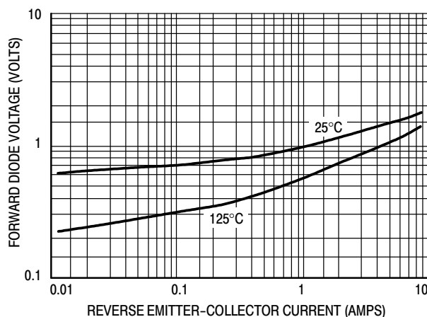
Figure 10. Forward Diode Voltage
