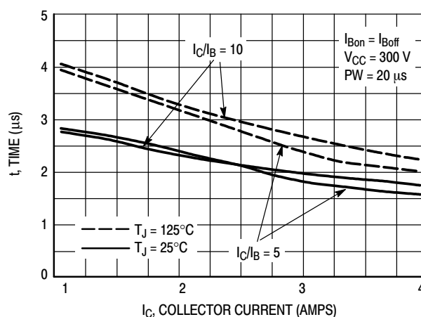
Figure 14. Resistive Switch Time, t_{off}
