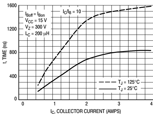
Figure 19. Inductive Switching, t_t @ I_C/I_B = 10
