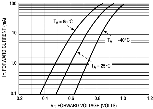
Figure 1. Forward Voltage
