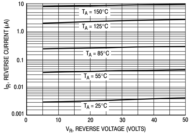
Figure 2. Leakage Current
