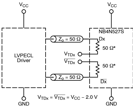
Figure 7. LVPECL Interface
