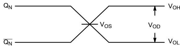
Figure 15. LVDS Output
