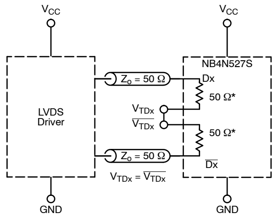
Figure 8. LVDS Interface
