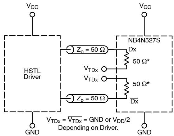
Figure 10. HSTL Interface
