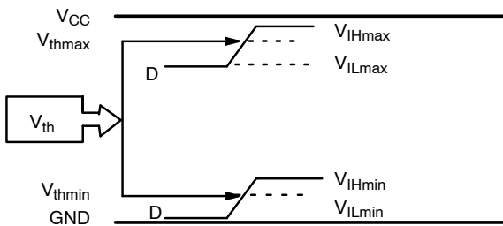
Figure 18. V_{th} Diagram
