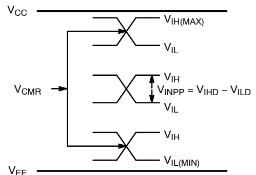
Figure 19. V_{CMR} Diagram
