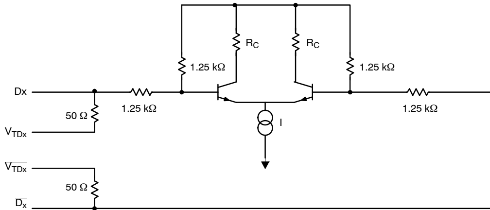
Figure 6. Input Structure
