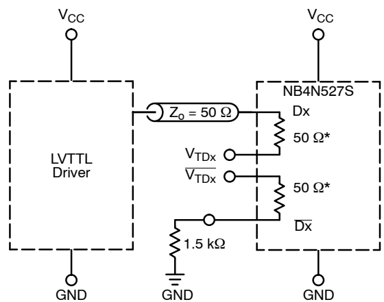
Figure 12. LVTTTL Interface
