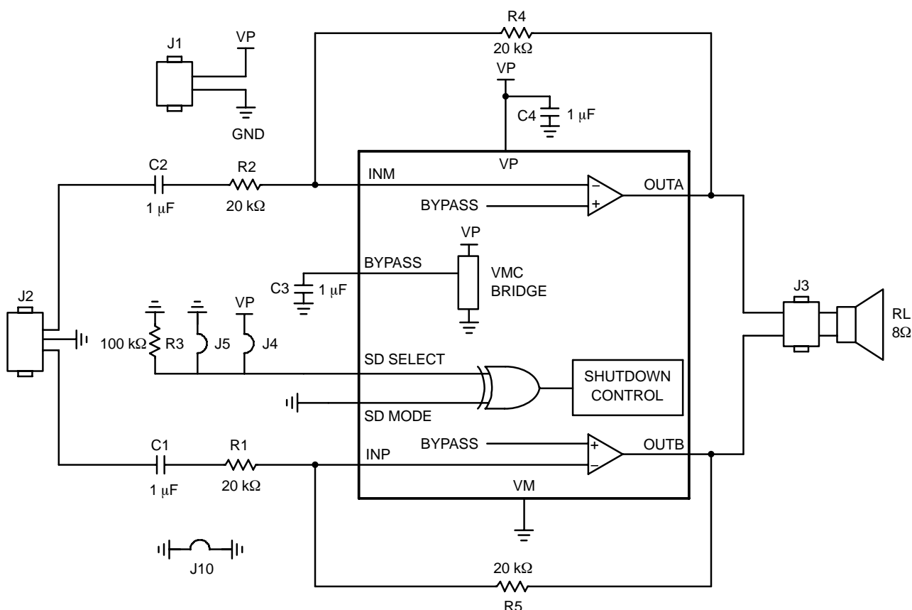
Figure 31. Demonstration Board Schematic
