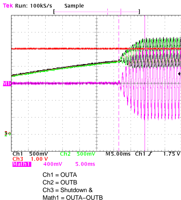
Figure 22. Turning-on Sequence Zoom @ VP = 5 V and f = 1 kHz
