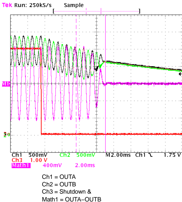
Figure 24. Turning-off Sequence Zoom @ VP = 5 V and f = 1 kHz
