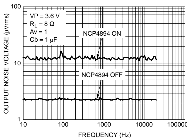
Figure 19. Noise Floor @ VP = 3.6 V
