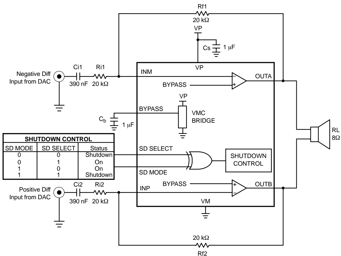
Figure 1. Typical NCP4894 Application Circuit with Differential Input
