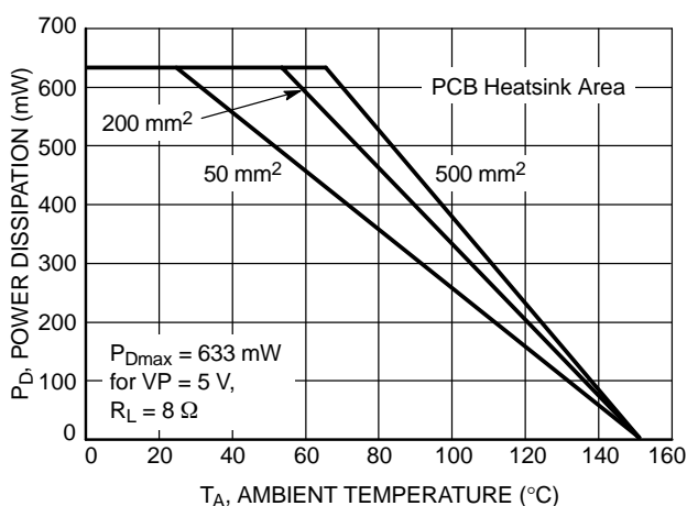
Figure 29. Power Derating – 9-Pin Flip-Chip CSP
