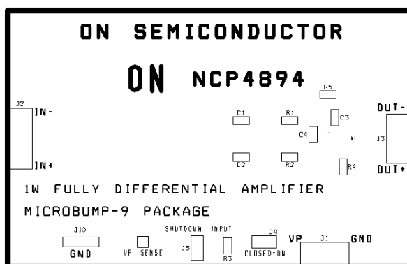
Silkscreen Layer
