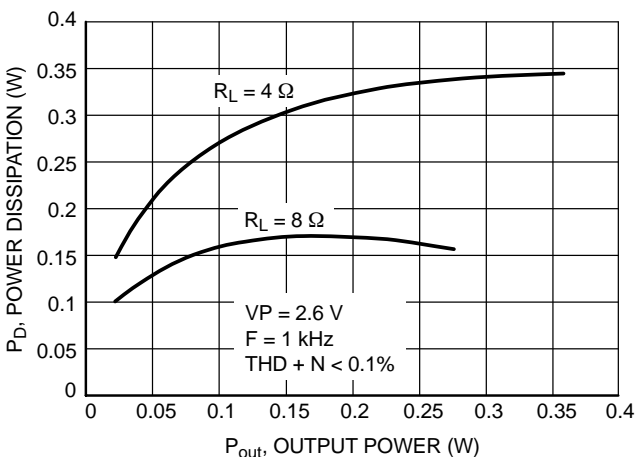
Figure 28. Power Dissipation versus Output Power
