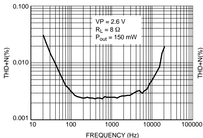
Figure 5. THD+N versus Frequency
