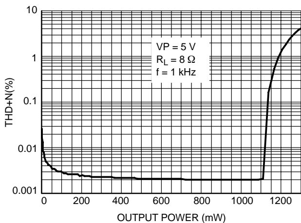
Figure 7. THD+N versus Output Power
