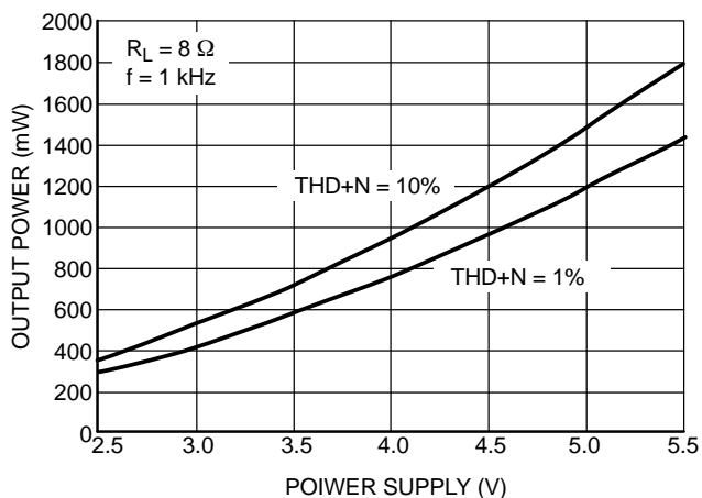
Figure 11. THD+N versus Output Power
