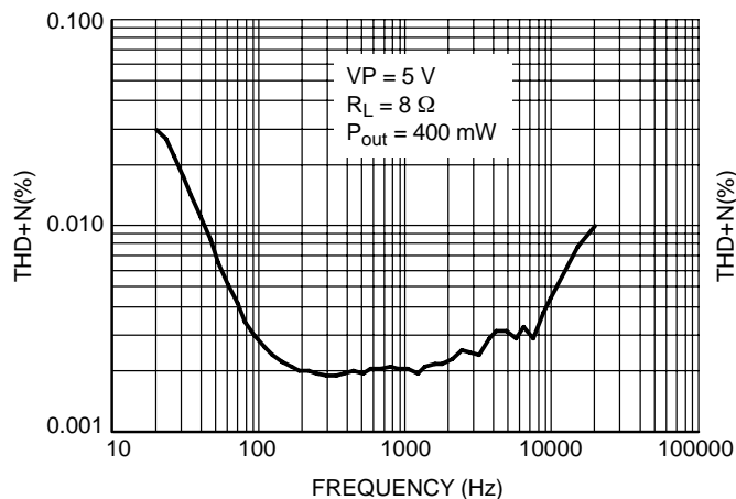
Figure 3. THD+N versus Frequency
