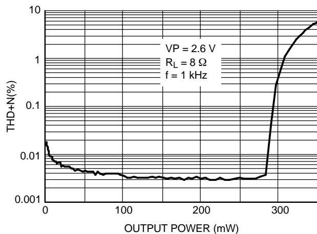
Figure 9. THD+N versus Output Power
