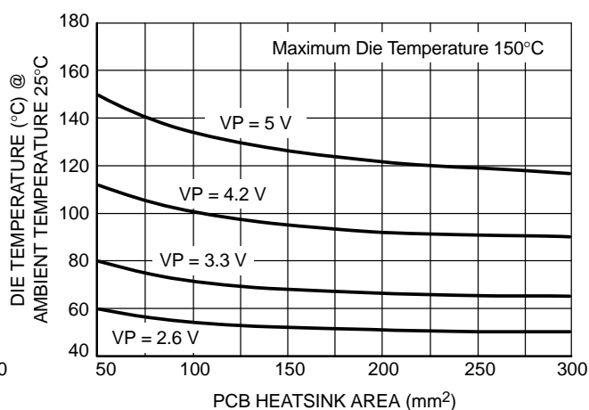
Figure 30. Maximum Die Temperature versus PCB Heatsink Area
