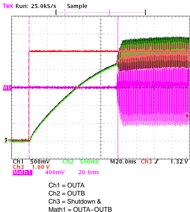
Figure 21. Turning-on Sequence @ VP = 5 V and f = 1 kHz
