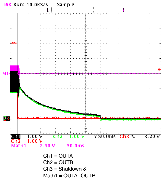
Figure 23. Turning-off Sequence @ VP = 5 V and f = 1 kHz
