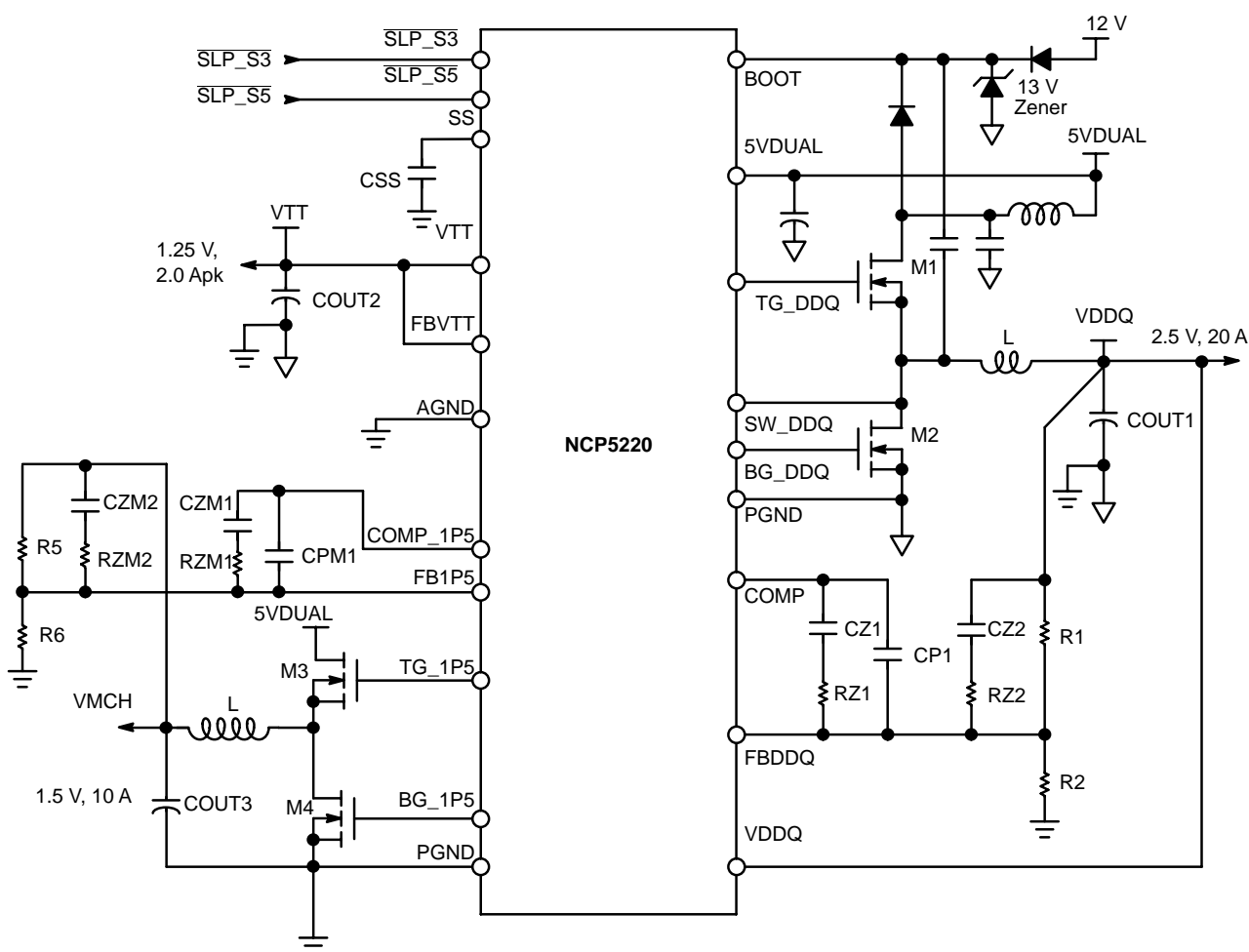
Figure 1. Application Diagram
