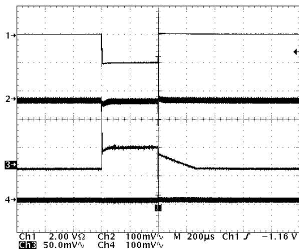
Channel 1: Current Sunk into VTT, 2.0 A/div Channel 2: VDDQ output Voltage, AC-Coupled, 100 mV/div Channel 3: VTT Output Voltage, AC-Coupled, 50 mV/div Channel 4: V1P5 Vutput Voltage, AC-Coupled, 100 mV/div Time Base: 200 \mu s/div
