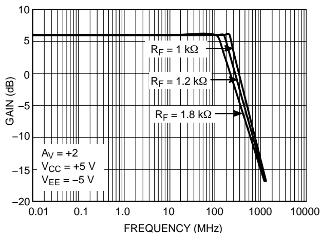
Figure 24. Frequency Response vs. R_F
