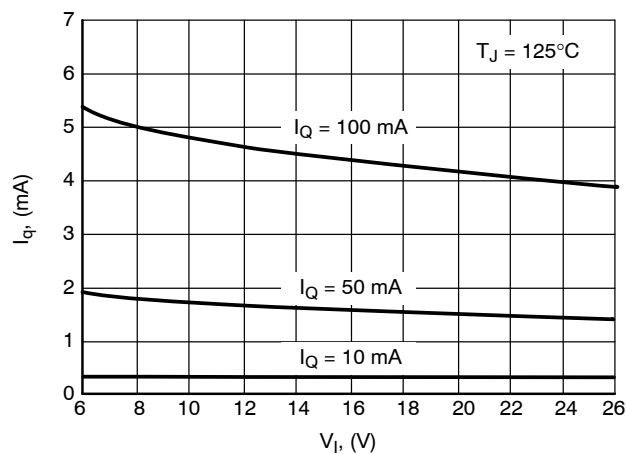
Figure 16. Quiescent Current I_q vs. Input Voltage V_I
