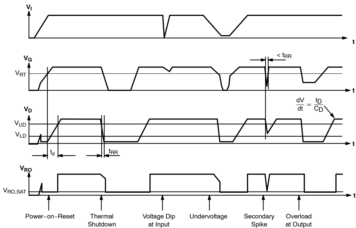
Figure 3. Reset Timing Diagram
