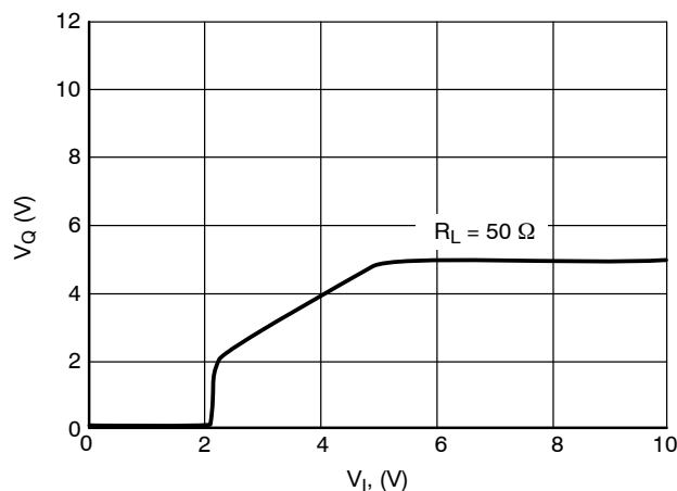
Figure 10. Output Voltage V_Q vs. Input Voltage V_I
