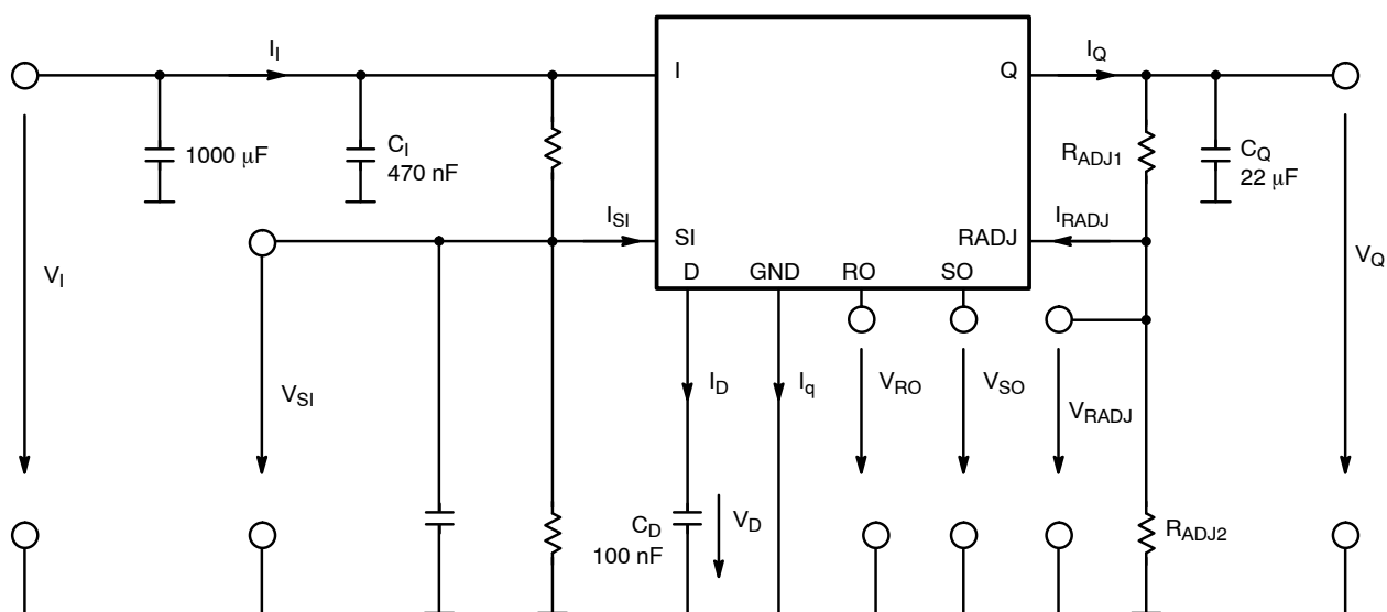
Figure 2. Measuring Circuit
