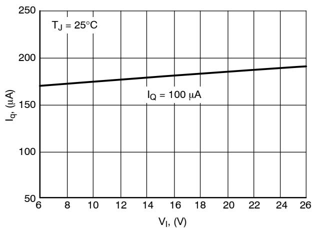
Figure 17. Quiescent Current I_q vs. Input Voltage V_I
