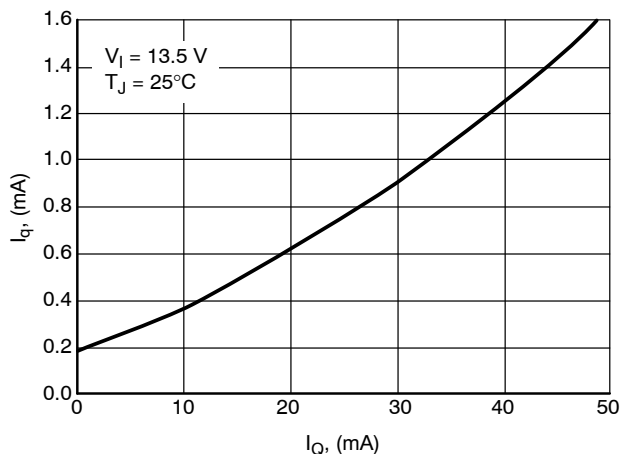
Figure 15. Current Consumption I_q vs. Output Current I_Q
