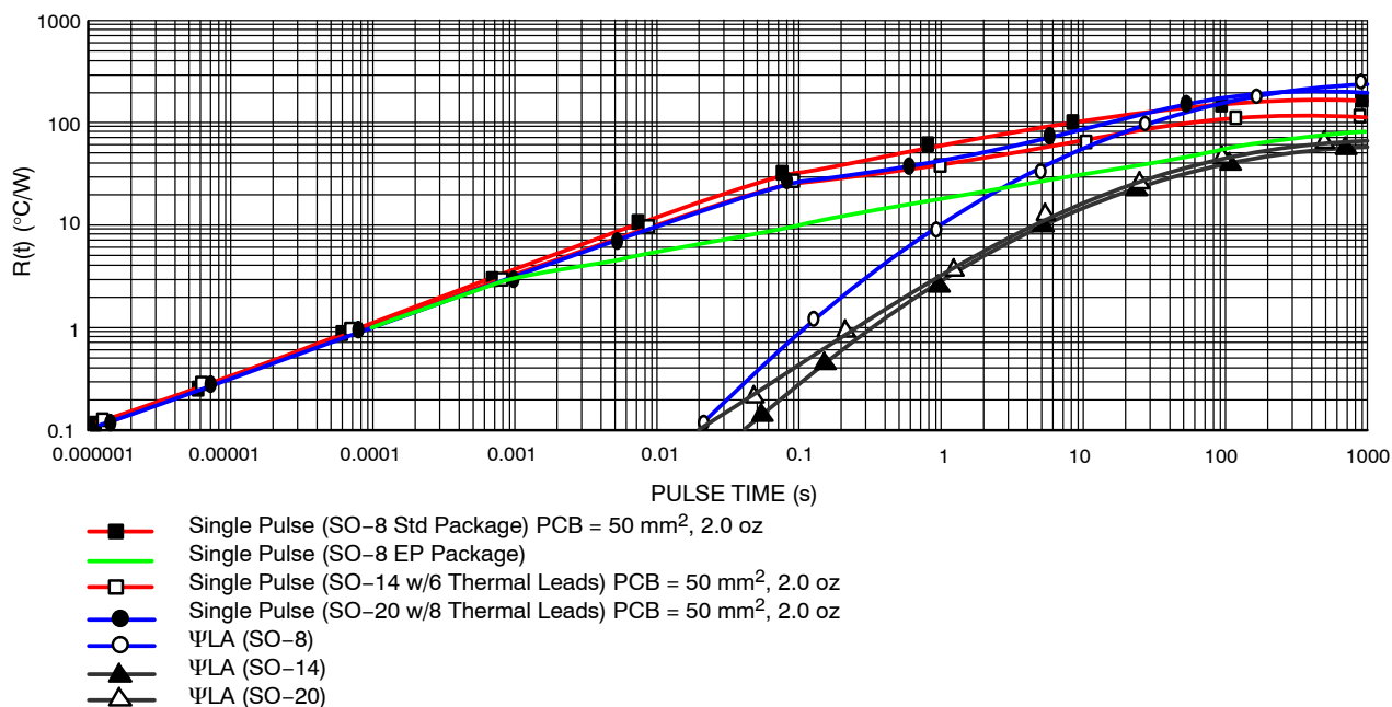
Figure 20. R(t) vs. Pulse Time
