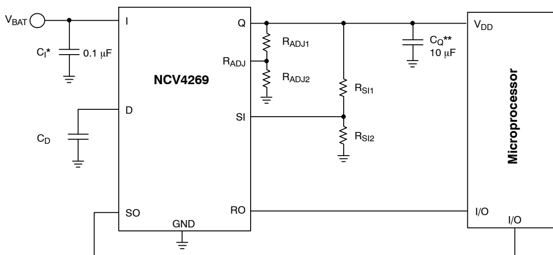
Figure 21. Application Diagram
