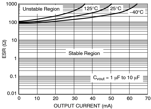
Figure 4. Output Stability
