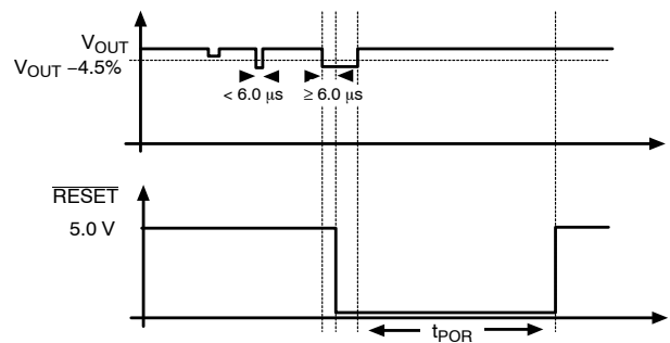
Figure 11. Undervoltage Triggered RESET
