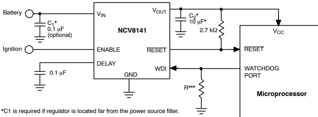
Figure 14. Application Diagram
