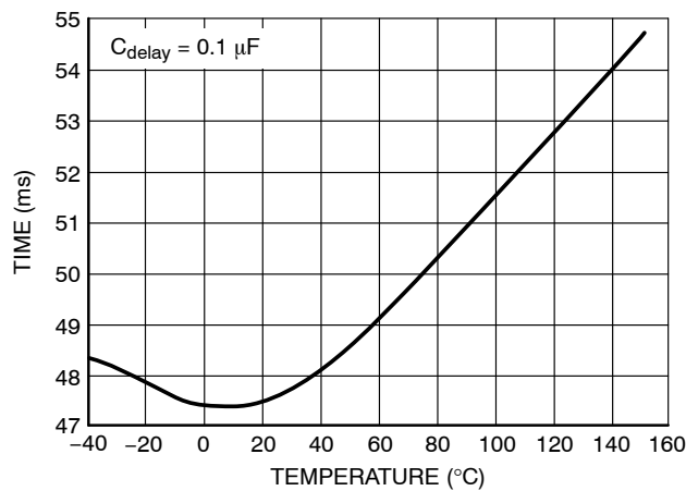
Figure 6. Delay Time
