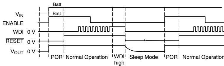
WDI Held High After a Normal Period of Operation; ENABLE = LOW
