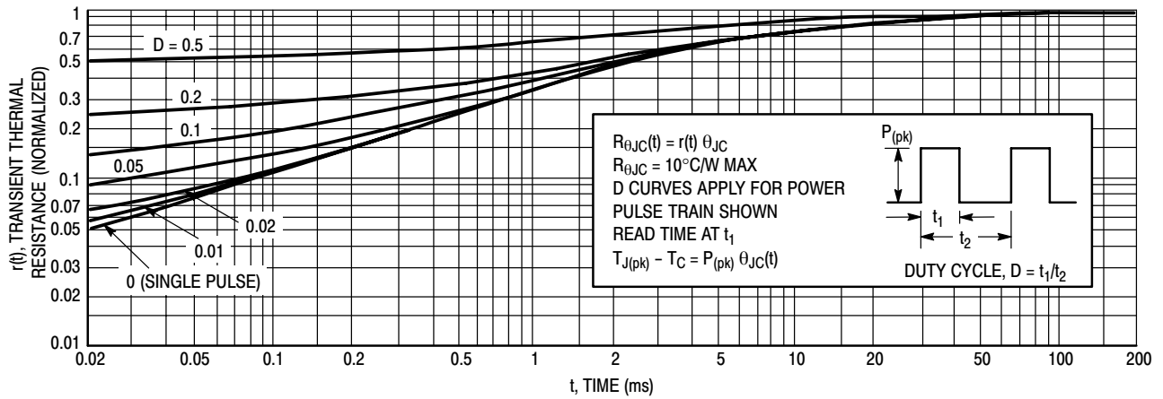
Figure 6. Thermal Response
