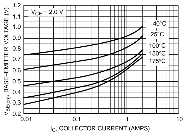
Figure 5. Base-Emitter Voltage
