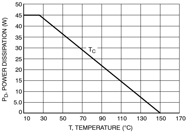
Figure 2. Power Derating
