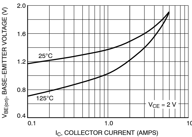
Figure 6. Base-Emitter Voltage
