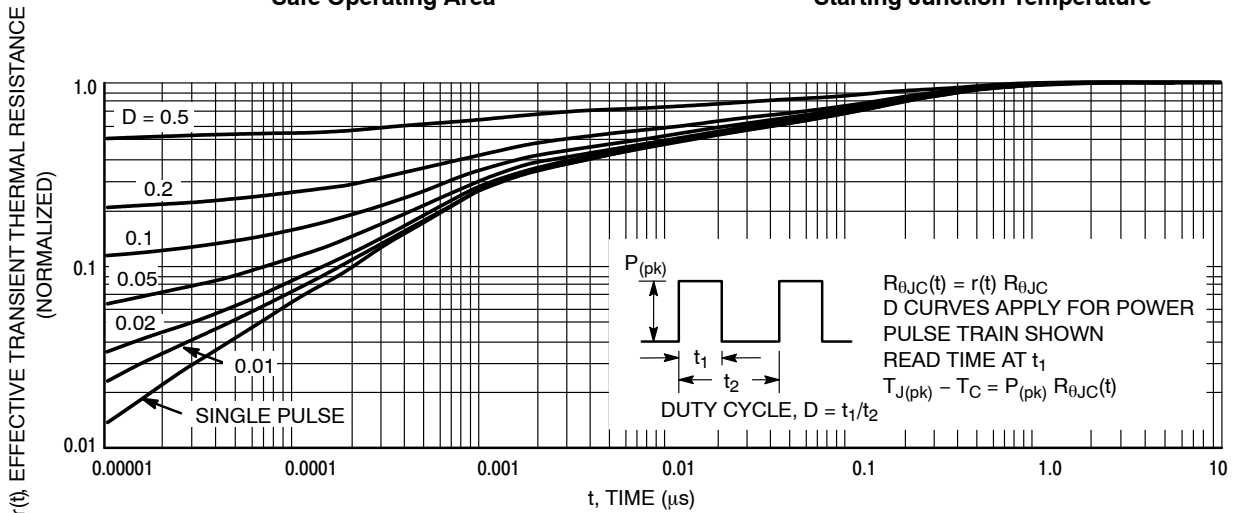
Figure 13. Thermal Response
