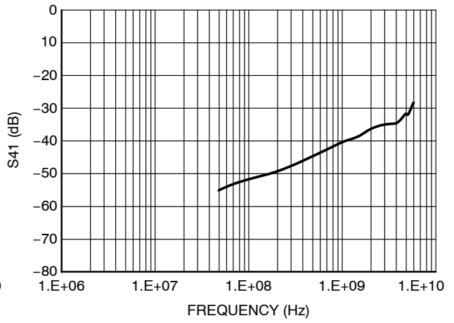
Figure 5. Analog Crosstalk
