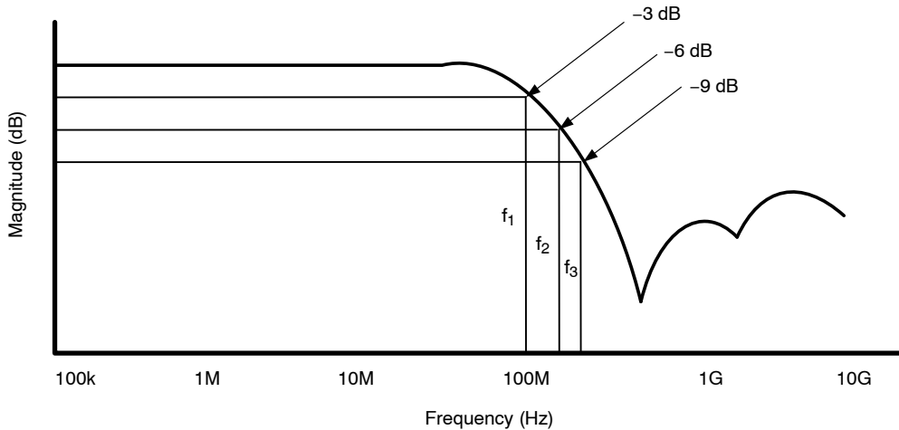
Figure 8. Filter Bandwidth
