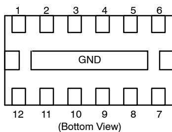
Figure 3. Pin Diagram
