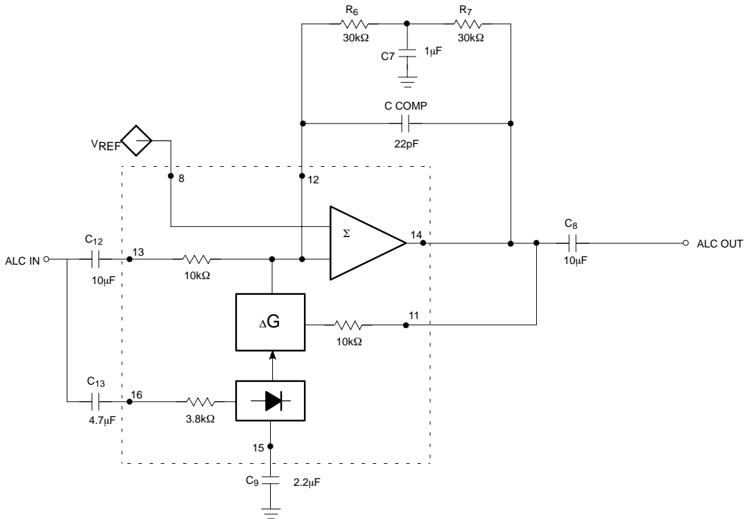
Figure 4. Typical ALC Configuration
