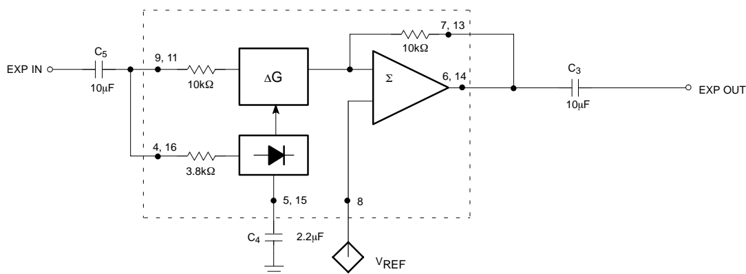
Figure 2. Typical Expander Configuration
