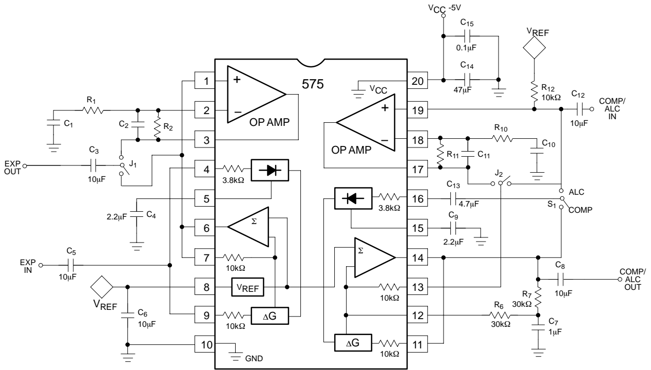
Figure 5. SA575 Low Voltage Expander/Compressor/ALC Demo Board
