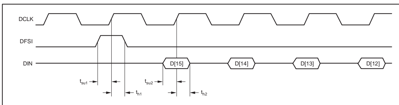
Figure 2. Input Data Interface Timing
