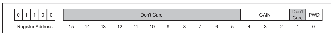
Figure 20. PGA and PWD Register
