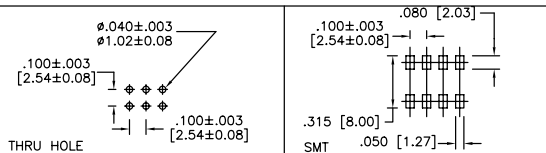
RECOMMENDED BOARD LAYOUT
