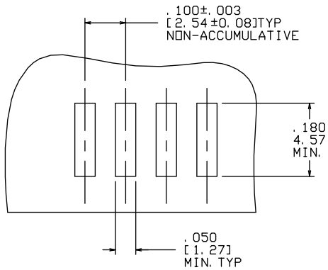
FIGURE A TOP ENTRY .025/.64 SQ PIN
