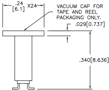
FIGURE 1 SMALL CAP FOR LESS THAN 6 POSITION
