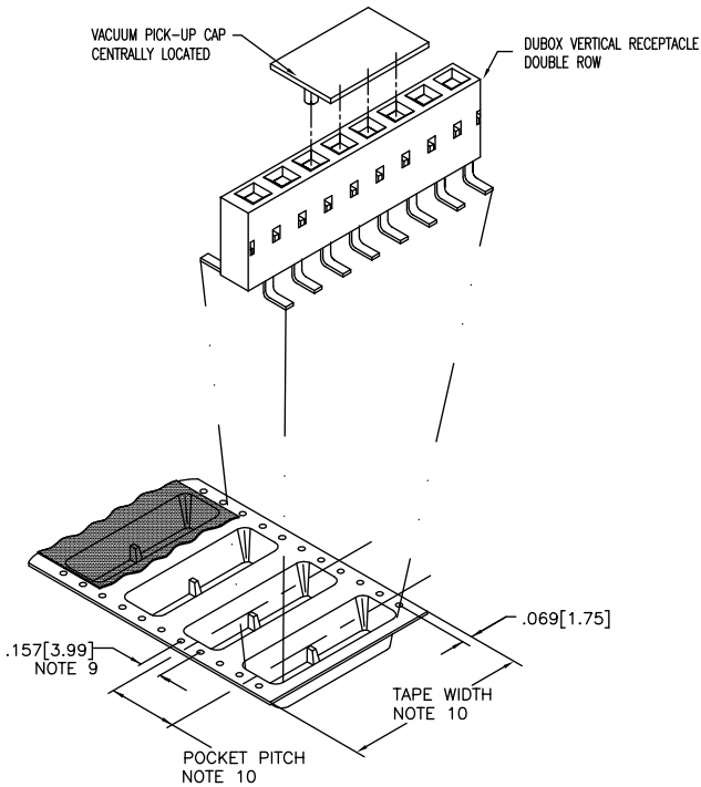
FIGURE 2 TAPE & REEL PACKAGING
