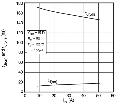
FIGURE 14, DELAY TIMES vs CURRENT
