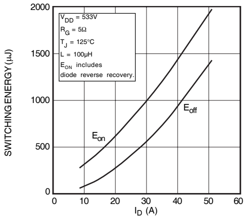
FIGURE 16, SWITCHING ENERGY vs CURRENT
