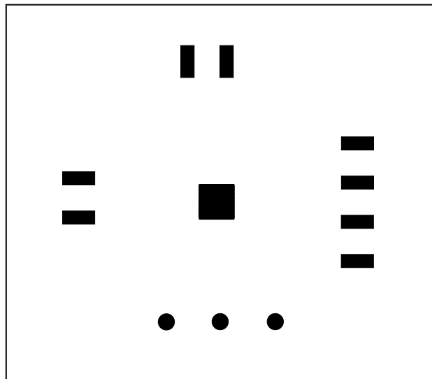
Figure 9. MAX9994 EV Kit PC Board Layout—Bottom Soldermask
