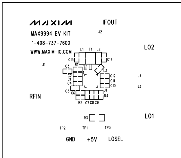
Figure 3. MAX9994 EV Kit PC Board Layout—Top Silkscreen
