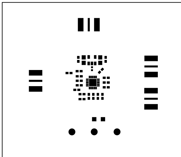
Figure 4. MAX9994 EV Kit PC Board Layout—Top Soldermask
