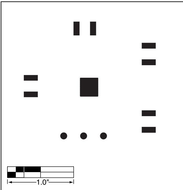
Figure 9. MAX9993 EV Kit PC Board Layout—Bottom Soldermask
