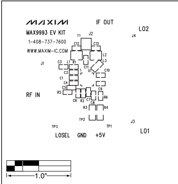
Figure 3. MAX9993 EV Kit PC Board Layout—Top Silkscreen
