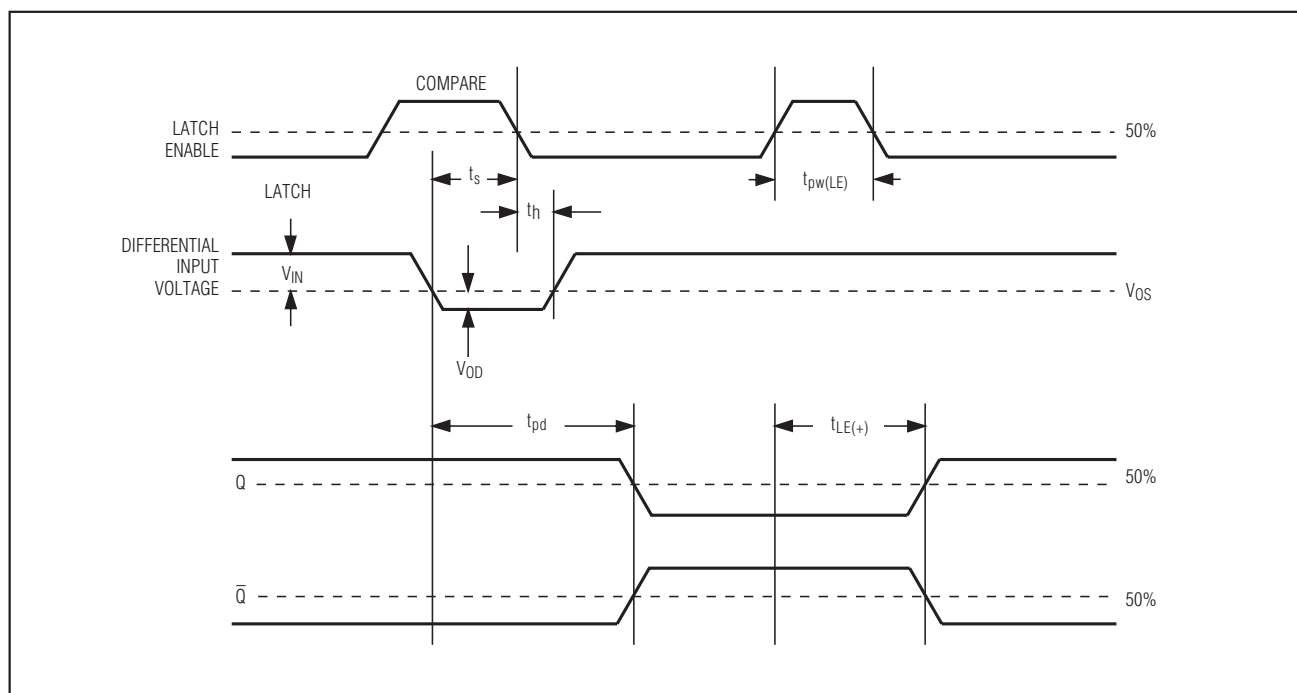
Figure 3. Timing Diagram
