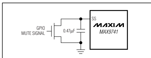
Figure 2. MAX9741 Mute Circuit
