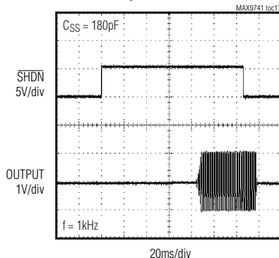
TURN-ON/TURN-OFF RESPONSE
