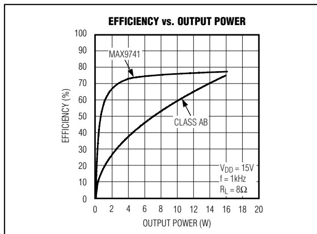
Figure 1. MAX9741 Efficiency vs. Class AB Efficiency
