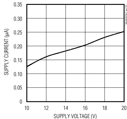
SHUTDOWN SUPPLY CURRENT vs. SUPPLY VOLTAGE
