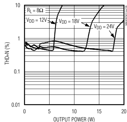
TOTAL HARMONIC DISTORTION PLUS NOISE vs. OUTPUT POWER WITH FERRITE BEAD FILTER
