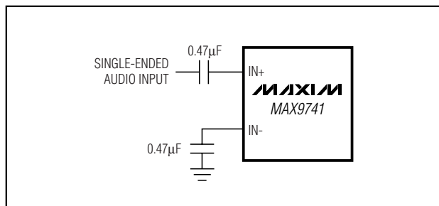
Figure 4. Single-Ended Input
