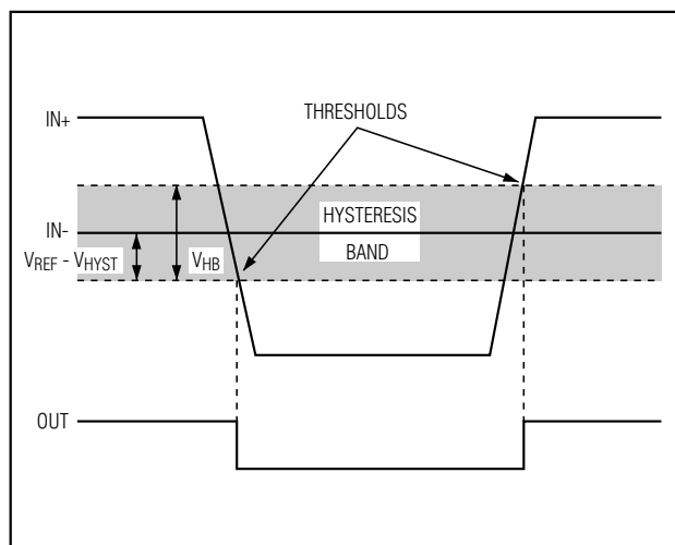
Figure 2. Threshold Hysteresis Band
