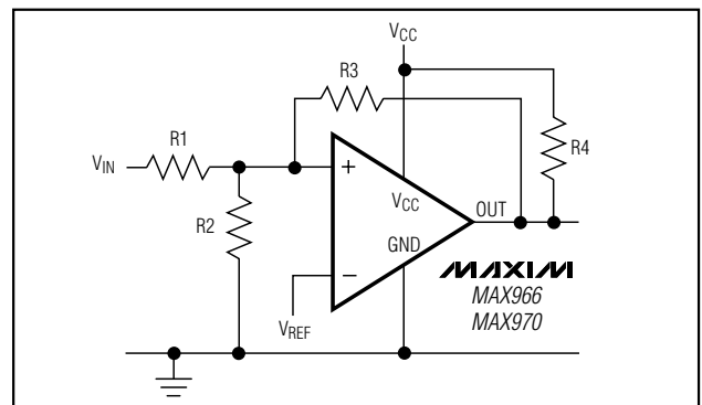
Figure 4. External Hysteresis
