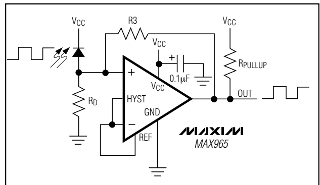
Figure 5. IR Receiver
