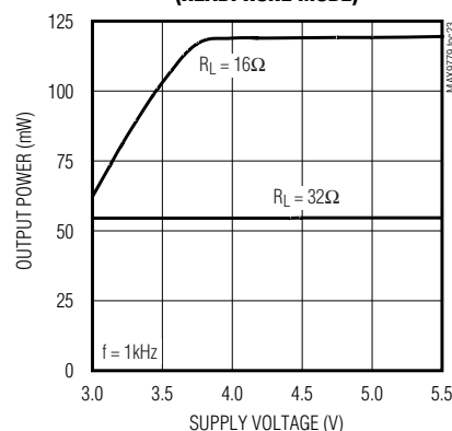
OUTPUT POWER vs. SUPPLY VOLTAGE (HEADPHONE MODE)
