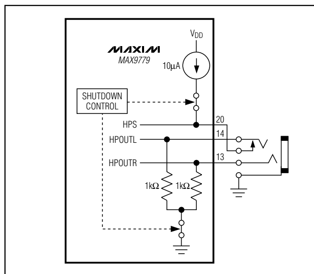
Figure 5. HPS Configuration
