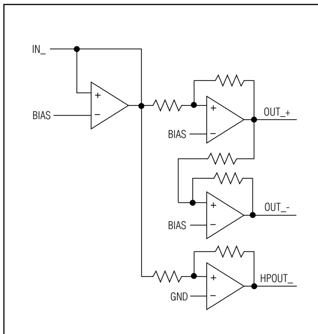
Figure 1. MAX9779 Signal Path
