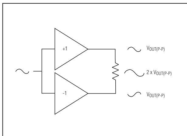
Figure 6. Bridge-Tied Load Configuration
