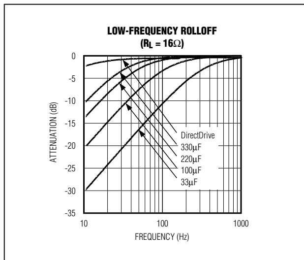
Figure 3. Low-Frequency Attenuation of Common DC-Blocking Capacitor Values
