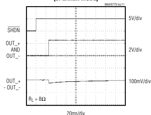
TURN-ON RESPONSE (SPEAKER MODE)
