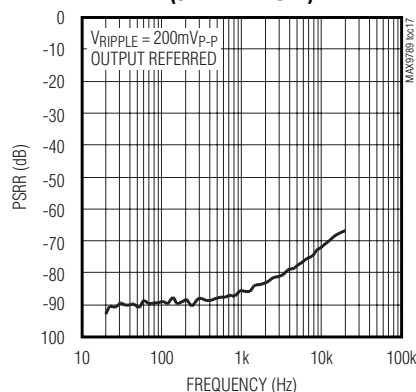
POWER-SUPPLY REJECTION RATIO (SPEAKER MODE)
