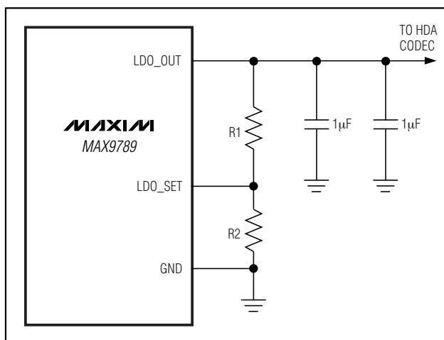
Figure 1. Adjustable Output Using External Feedback Resistors.
