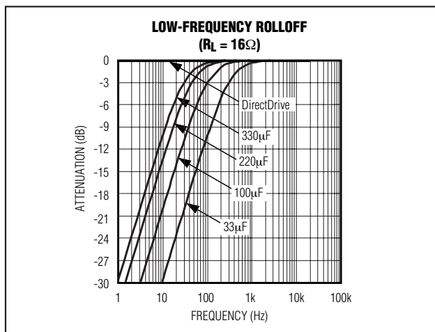
Figure 2. Low-Frequency Attenuation of Common DC-Blocking Capacitor Values
