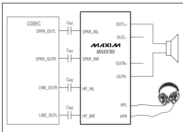
Figure 6. Mono Signal Output Configuration for MAX9789
