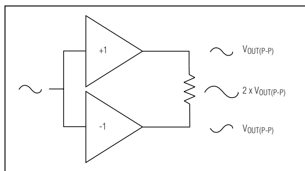
Figure 5. Bridge-Tied Load Configuration
