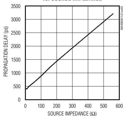
PROPAGATION DELAY vs. SOURCE IMPEDANCE
