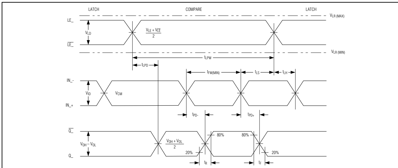
Figure 1. MAX9600/MAX9601/MAX9602 Timing Diagram
