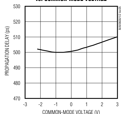
PROPAGATION DELAY vs. COMMON-MODE VOLTAGE
