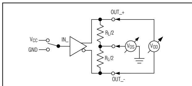
Figure 1. Driver V OD and V OS Test Circuit
