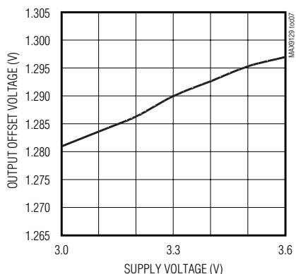
OUTPUT OFFSET VOLTAGE vs. SUPPLY VOLTAGE
