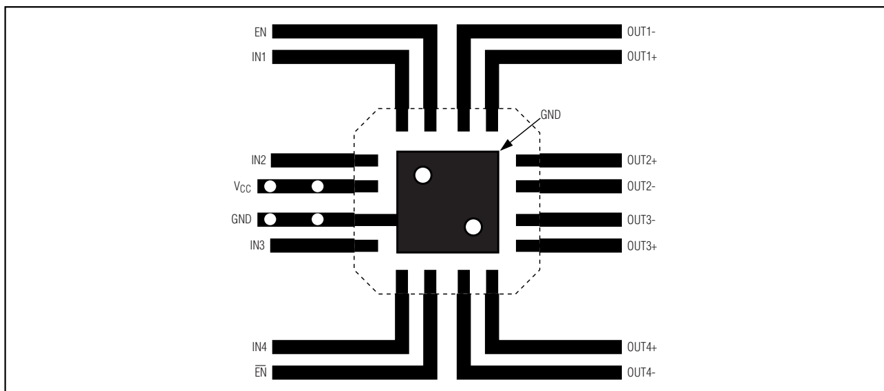
Figure 6. Suggested Layout for QFN Package
