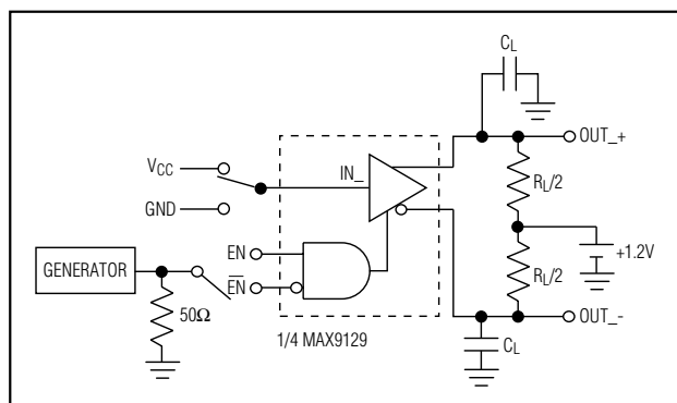
Figure 4. Driver High-Impedance Delay Test Circuit
