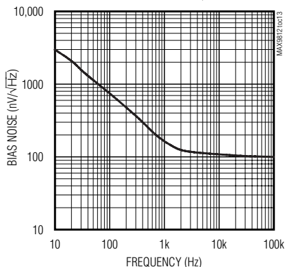
BIAS NOISE vs. FREQUENCY
