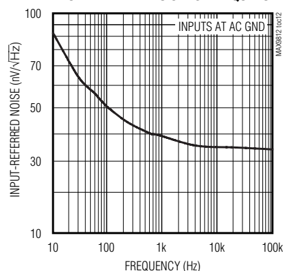
INPUT-REFERRED NOISE vs. FREQUENCY
