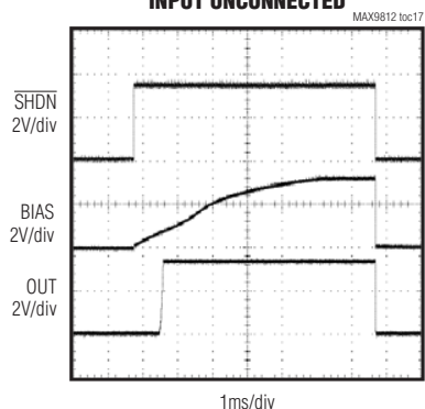
OUT-OF-SHUTDOWN WAVEFORM INPUT UNCONNECTED
