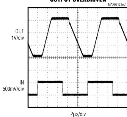
OUTPUT OVERDRIVEN
