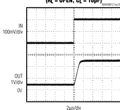
LARGE-SIGNAL PULSE RESPONSE ( R_L = OPEN , C_L = 10pF )
