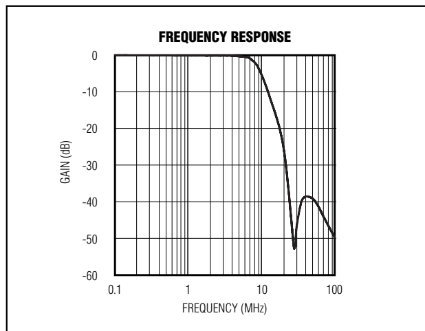
Figure 6. Frequency Response for 3rd-Order Lowpass Filter
