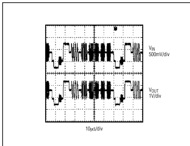
Figure 5. Multiburst Response
