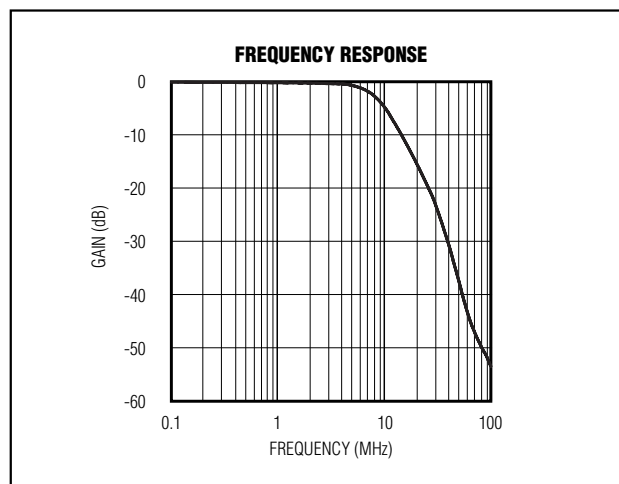
Figure 4. Frequency Response for 2nd-Order Lowpass Filter
