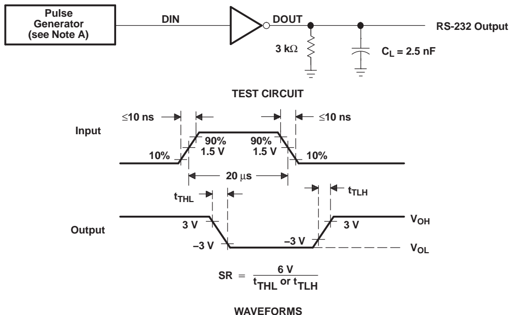
Figure 3. Test Circuit and Waveforms for t_{THL} and t_{TLH} Measurements (20-µs Input)
