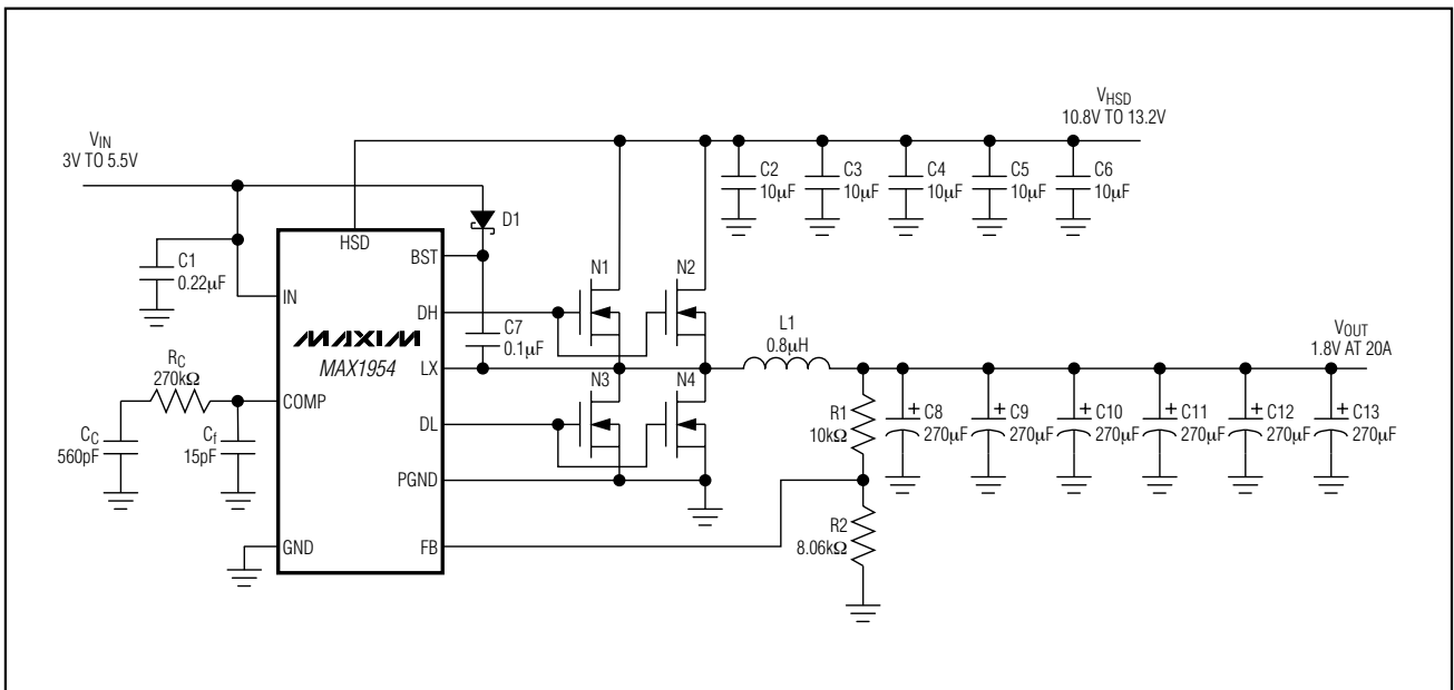
Figure 4. 20A Circuit
