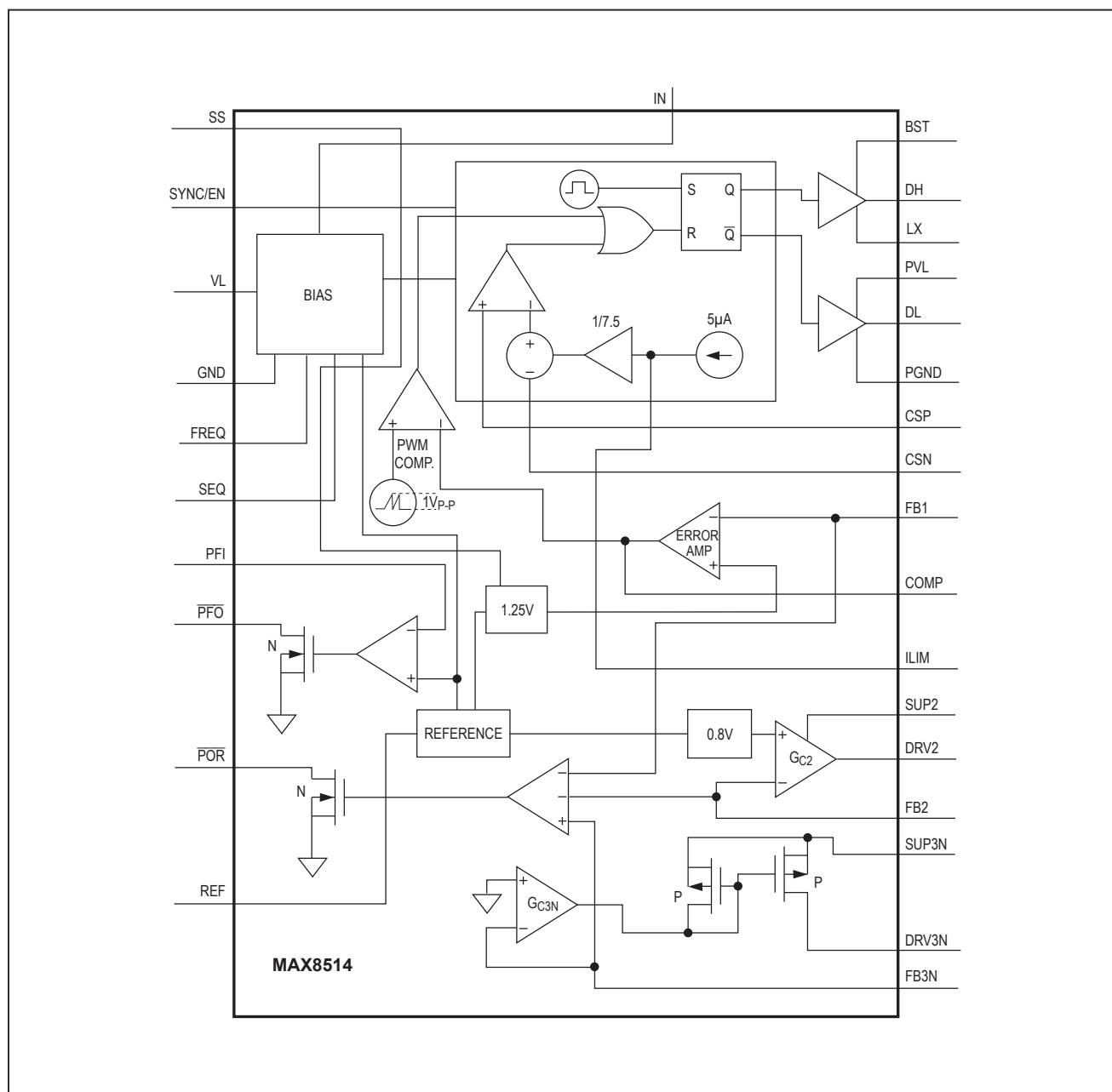
Figure 2. MAX8514 Functional Diagram
