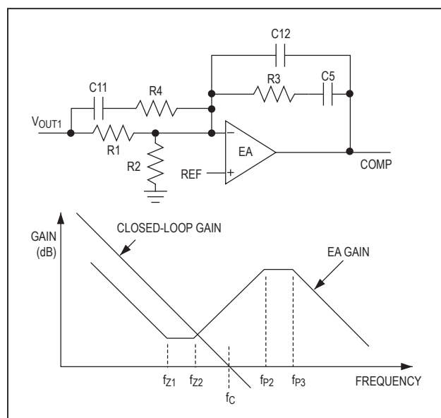
Figure 3. Case 1: Error-Amplifier Compensation Circuit (Closed-Loop and Error-Amplifier Gain Plot)
