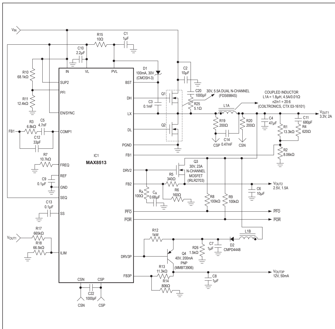
Figure 5. MAX8513 Typical Applications Circuit
