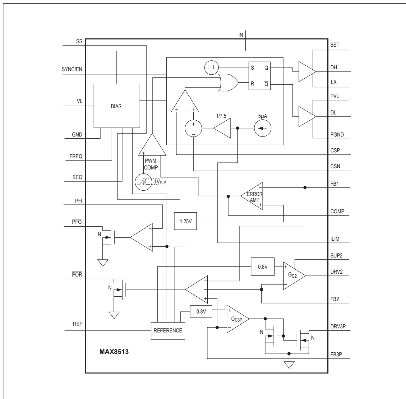
Figure 1. MAX8513 Functional Diagram
