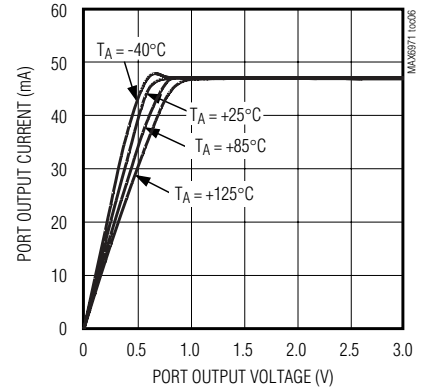
PORT OUTPUT CURRENT vs. PORT OUTPUT VOLTAGE ( R_{SET} = 360\Omega , V_+ = 3.3V )
