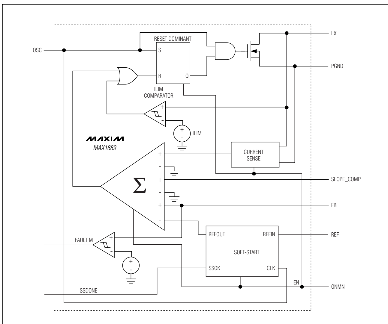
Figure 3. Main Step-Up Regulator Functional Diagram
