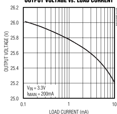
POSITIVE CHARGE-PUMP OUTPUT VOLTAGE vs. LOAD CURRENT
