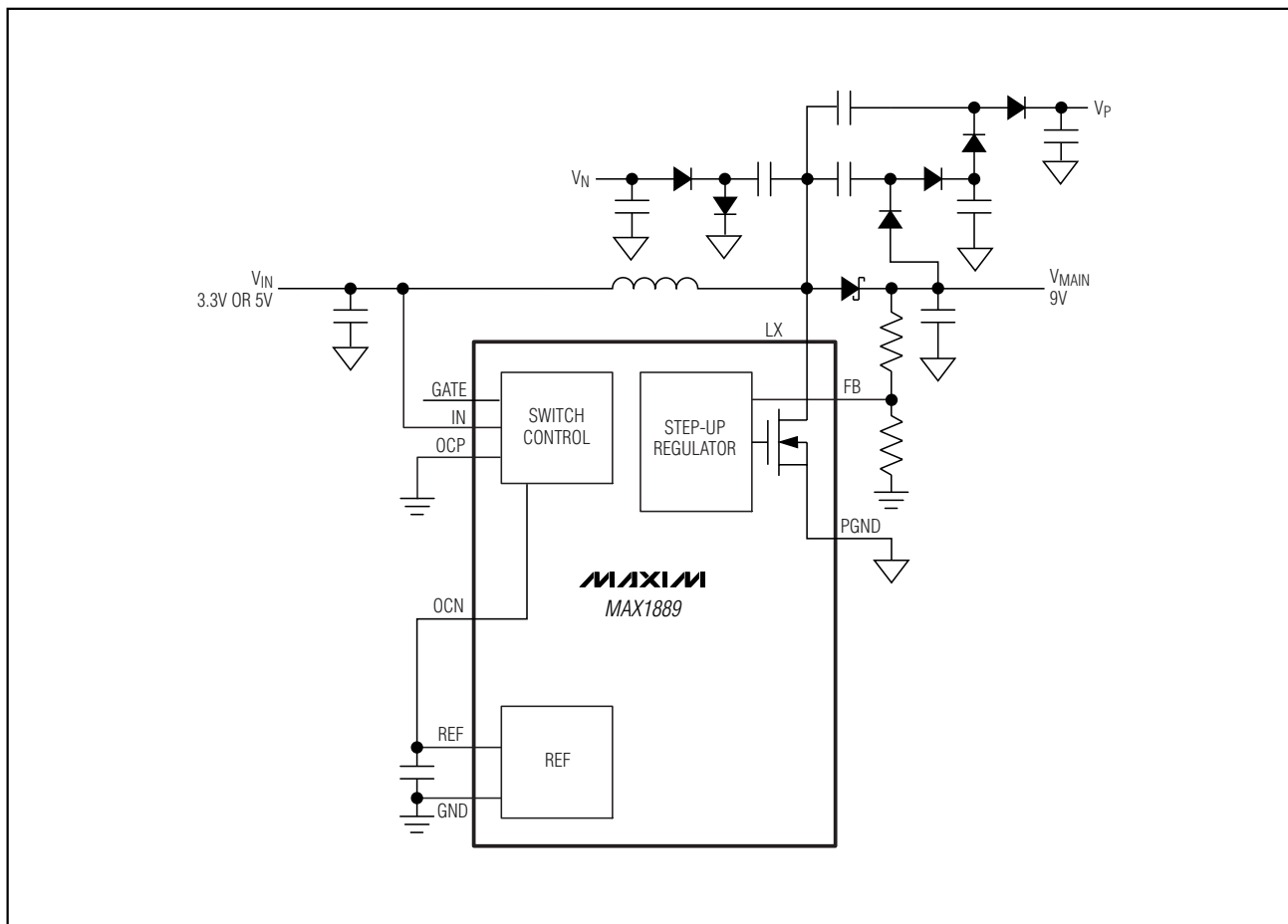
Figure 11. Disabling Input Protection MOSFET Switch
