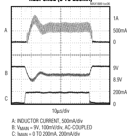
STEP-UP REGULATOR LOAD-TRANSIENT RESPONSE (0 TO 200mA)
