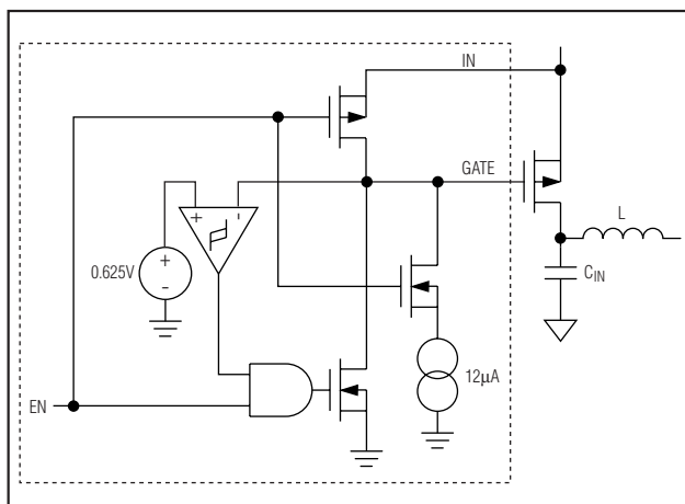
Figure 4. External Input P-Channel MOSFET Switch Control
