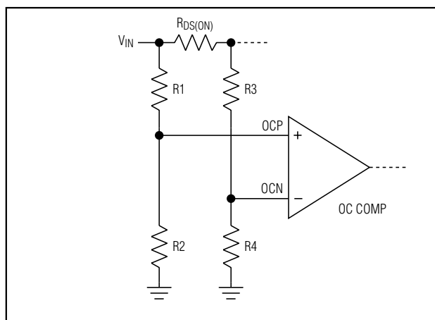
Figure 6. Setting the Overcurrent Threshold
