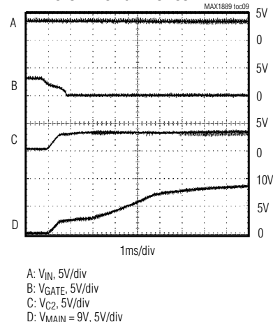
STEP-UP REGULATOR SOFT-START (200mA LOAD) FROM SLOW-RISING INPUT SUPPLY
