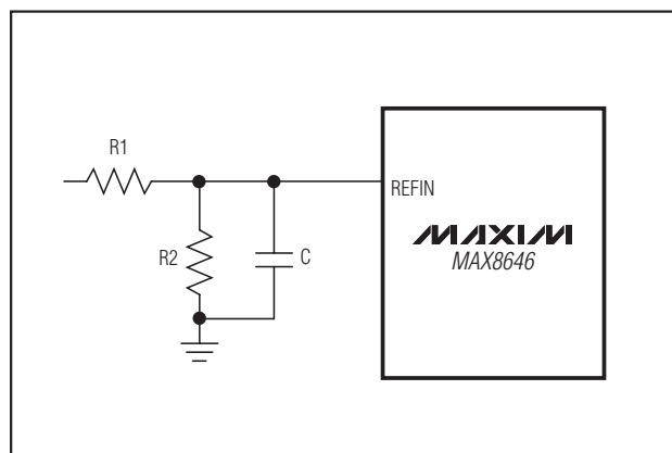
Figure 2. Typical Soft-Start Implementation with External Reference
