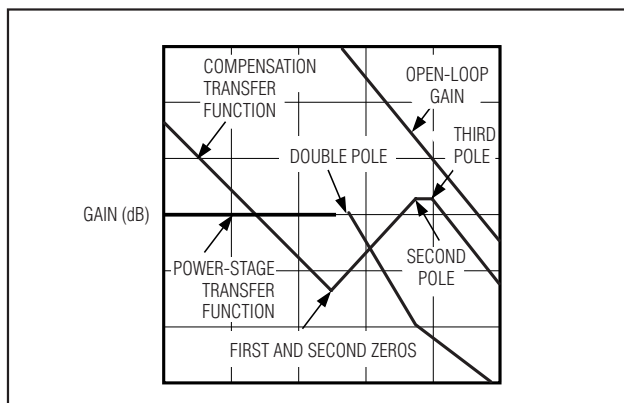
Figure 4. Type III Compensation Illustration
