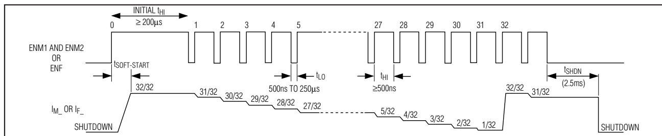
Figure 2. ENM1 and ENF Timing Diagram
