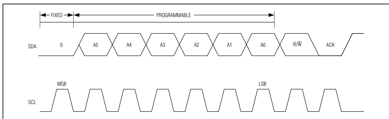
Figure 6. Slave Address
