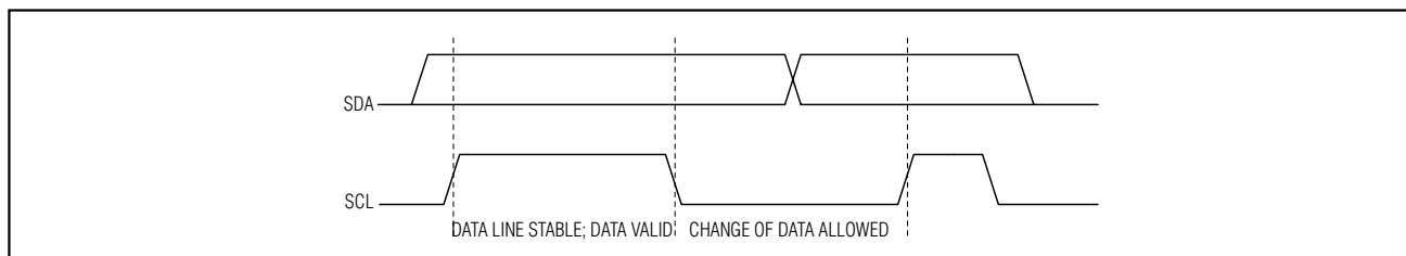
Figure 4. Bit Transfer
