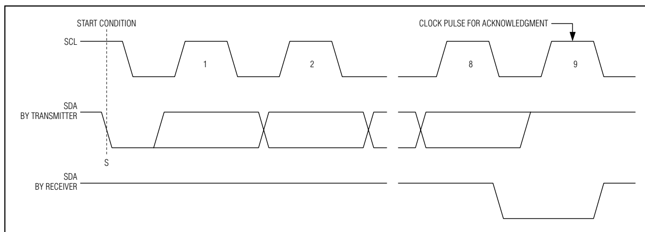
Figure 5. Acknowledge
