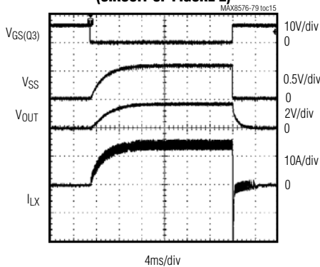
STARTUP AND SHUTDOWN (CIRCUIT OF FIGURE 2)
