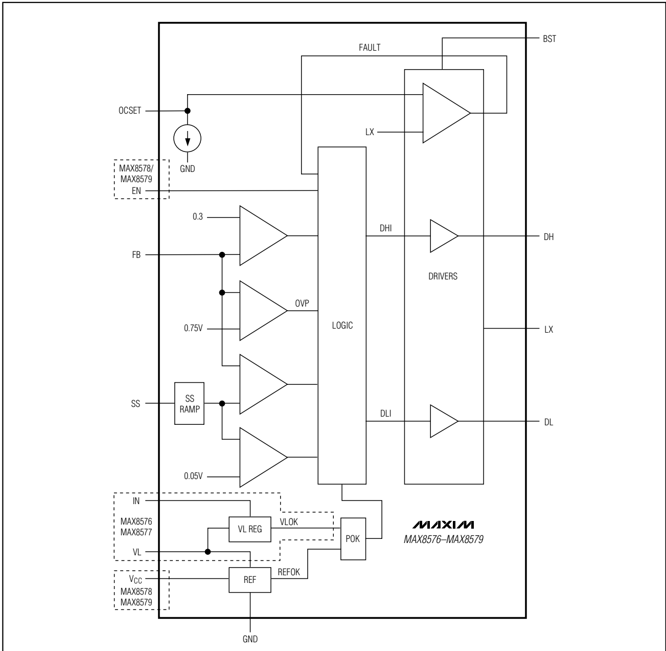
Figure 1. Functional Diagram
