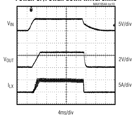
POWER-UP/POWER-DOWN WAVEFORMS
