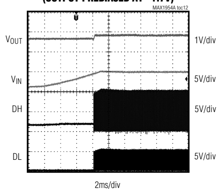
STARTUP INTO PREBIASED OUTPUT (OUTPUT PREBIASED AT ~1.7V)
