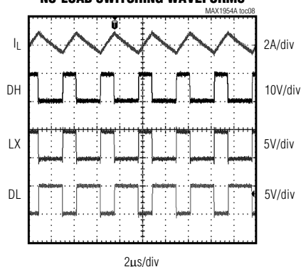
NO-LOAD SWITCHING WAVEFORMS
