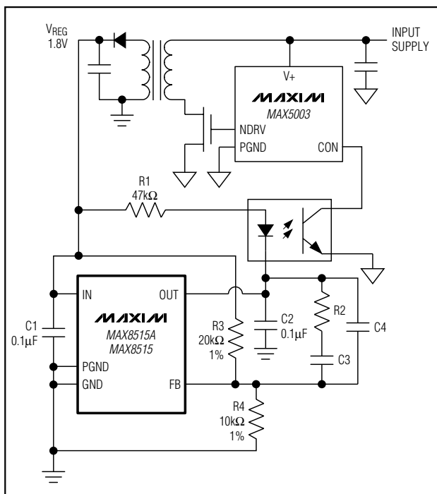
Figure 3. MAX8515A/MAX8515 Typical Application Circuit, Opto-Feedback Circuit
