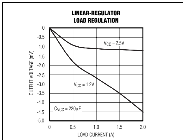
Figure 6. Load Regulation of Linear-Regulator Circuit
