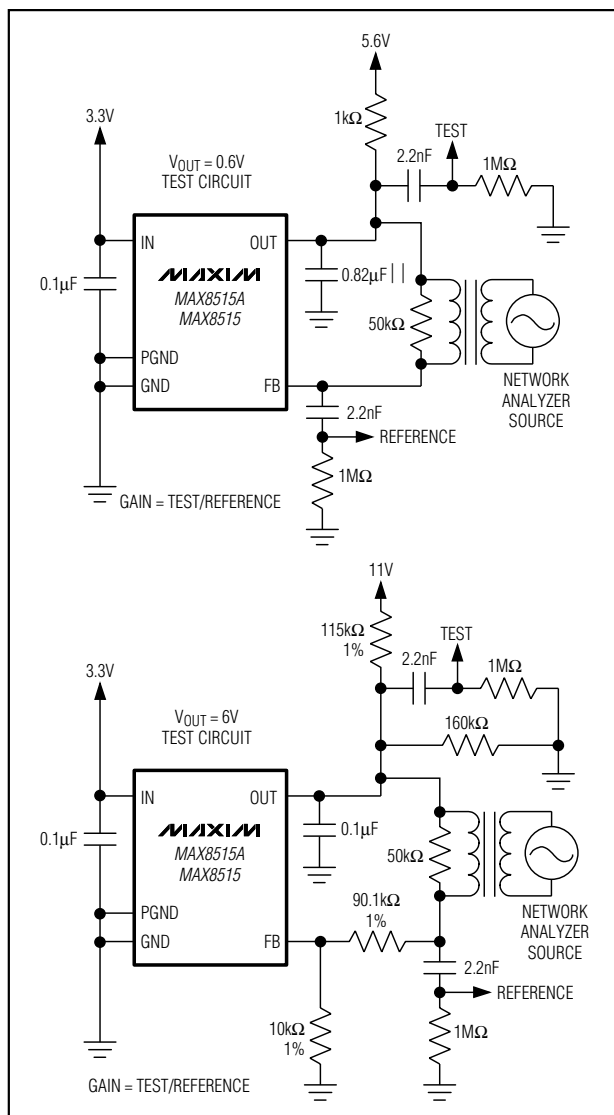
Figure 2. Test Circuits for Gain and Phase Plots
