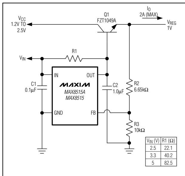
Figure 5. MAX8515A/MAX8515 Typical Application Circuit, Linear Regulator
